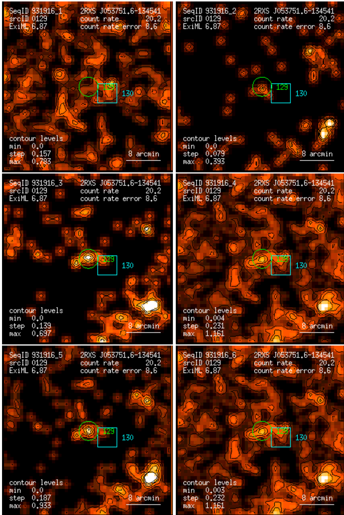
Figure 129: RASS 931916: detection 0129: band rate images, Gaussian filter: (1) PSPC channels 11 – 41, (2) 52 – 90, (3) 91 – 201, (4) 11 – 235, (5) 52 – 201, (6) 11 – 201. Broad band rates in counts/ks. Band rate contour levels in counts/ks/arcmin 2 .
