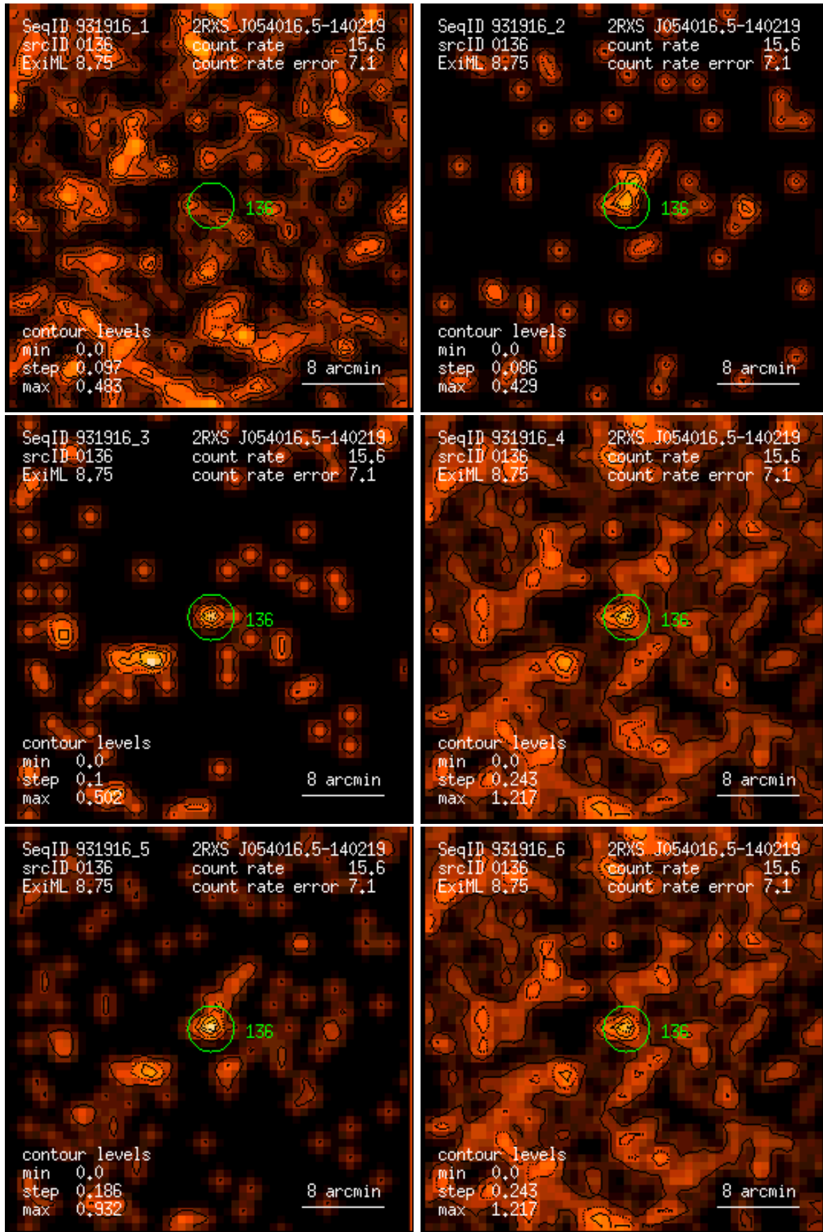
Figure 136: RASS 931916: detection 0136: band rate images, Gaussian filter: (1) PSPC channels 11 – 41, (2) 52 – 90, (3) 91 – 201, (4) 11 – 235, (5) 52 – 201, (6) 11 – 201. Broad band rates in counts/ks. Band rate contour levels in counts/ks/arcmin 2 .
