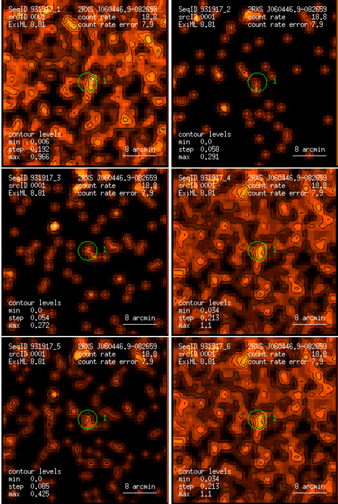
Figure 1: RASS 931917: detection 0001: band rate images, Gaussian filter: (1) PSPC channels 11 – 41, (2) 52 – 90, (3) 91 – 201, (4) 11 – 235, (5) 52 – 201, (6) 11 – 201. Broad band rates in counts/ks. Band rate contour levels in counts/ks/arcmin 2 .
