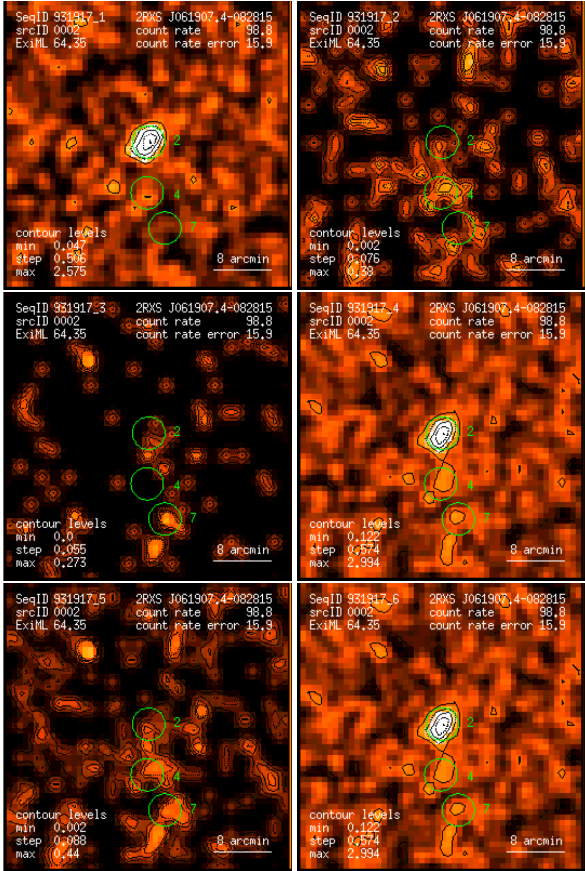
Figure 2: RASS 931917: detection 0002: band rate images, Gaussian filter: (1) PSPC channels 11 – 41, (2) 52 – 90, (3) 91 – 201, (4) 11 – 235, (5) 52 – 201, (6) 11 – 201. Broad band rates in counts/ks. Band rate contour levels in counts/ks/arcmin 2 .
