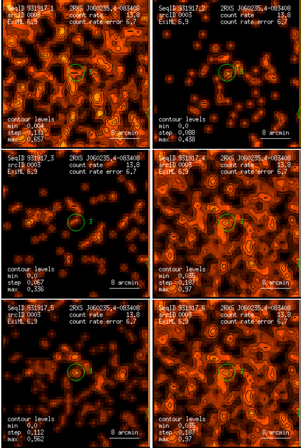
Figure 3: RASS 931917: detection 0003: band rate images, Gaussian filter: (1) PSPC channels 11 – 41, (2) 52 – 90, (3) 91 – 201, (4) 11 – 235, (5) 52 – 201, (6) 11 – 201. Broad band rates in counts/ks. Band rate contour levels in counts/ks/arcmin 2 .
