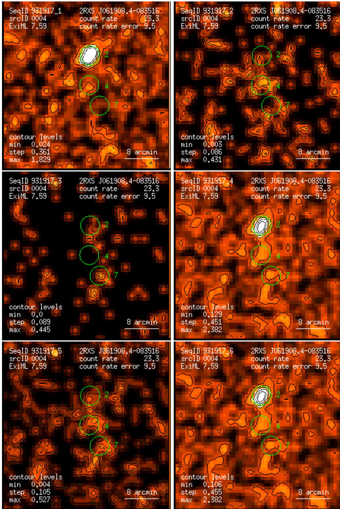
Figure 4: RASS 931917: detection 0004: band rate images, Gaussian filter: (1) PSPC channels 11 – 41, (2) 52 – 90, (3) 91 – 201, (4) 11 – 235, (5) 52 – 201, (6) 11 – 201. Broad band rates in counts/ks. Band rate contour levels in counts/ks/arcmin 2 .
