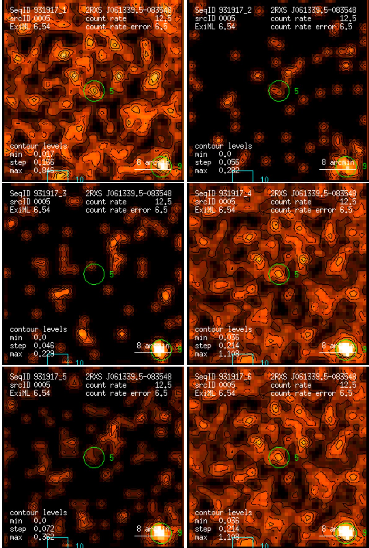
Figure 5: RASS 931917: detection 0005: band rate images, Gaussian filter: (1) PSPC channels 11 – 41, (2) 52 – 90, (3) 91 – 201, (4) 11 – 235, (5) 52 – 201, (6) 11 – 201. Broad band rates in counts/ks. Band rate contour levels in counts/ks/arcmin 2 .
