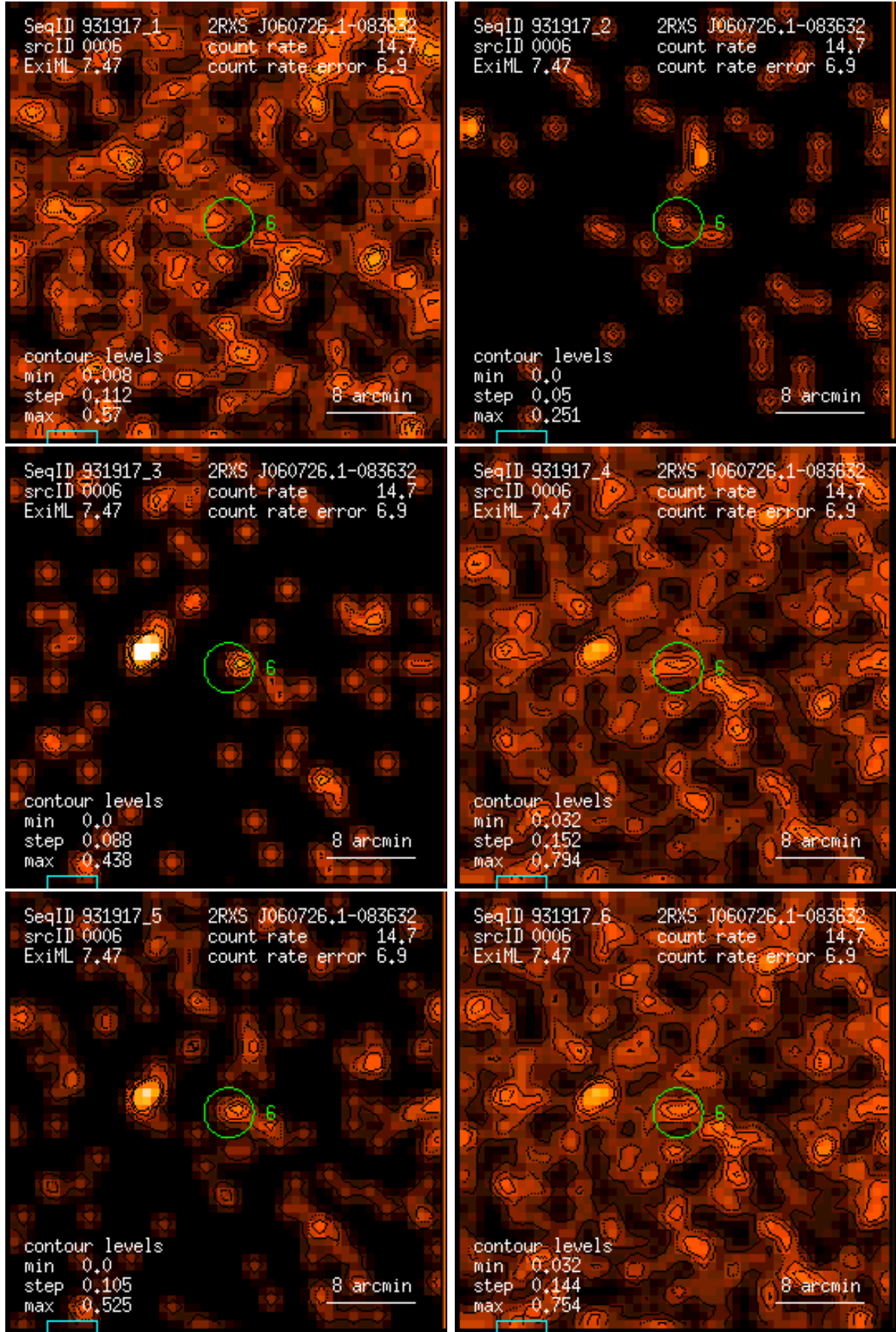
Figure 6: RASS 931917: detection 0006: band rate images, Gaussian filter: (1) PSPC channels 11 – 41, (2) 52 – 90, (3) 91 – 201, (4) 11 – 235, (5) 52 – 201, (6) 11 – 201. Broad band rates in counts/ks. Band rate contour levels in counts/ks/arcmin 2 .
