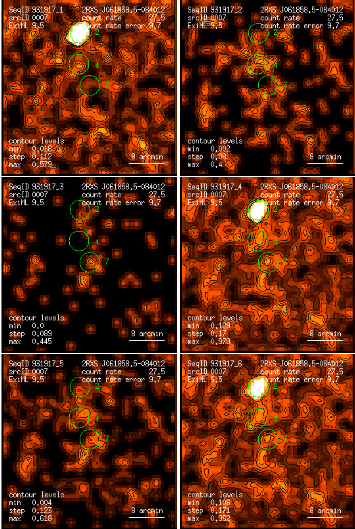
Figure 7: RASS 931917: detection 0007: band rate images, Gaussian filter: (1) PSPC channels 11 – 41, (2) 52 – 90, (3) 91 – 201, (4) 11 – 235, (5) 52 – 201, (6) 11 – 201. Broad band rates in counts/ks. Band rate contour levels in counts/ks/arcmin 2 .
