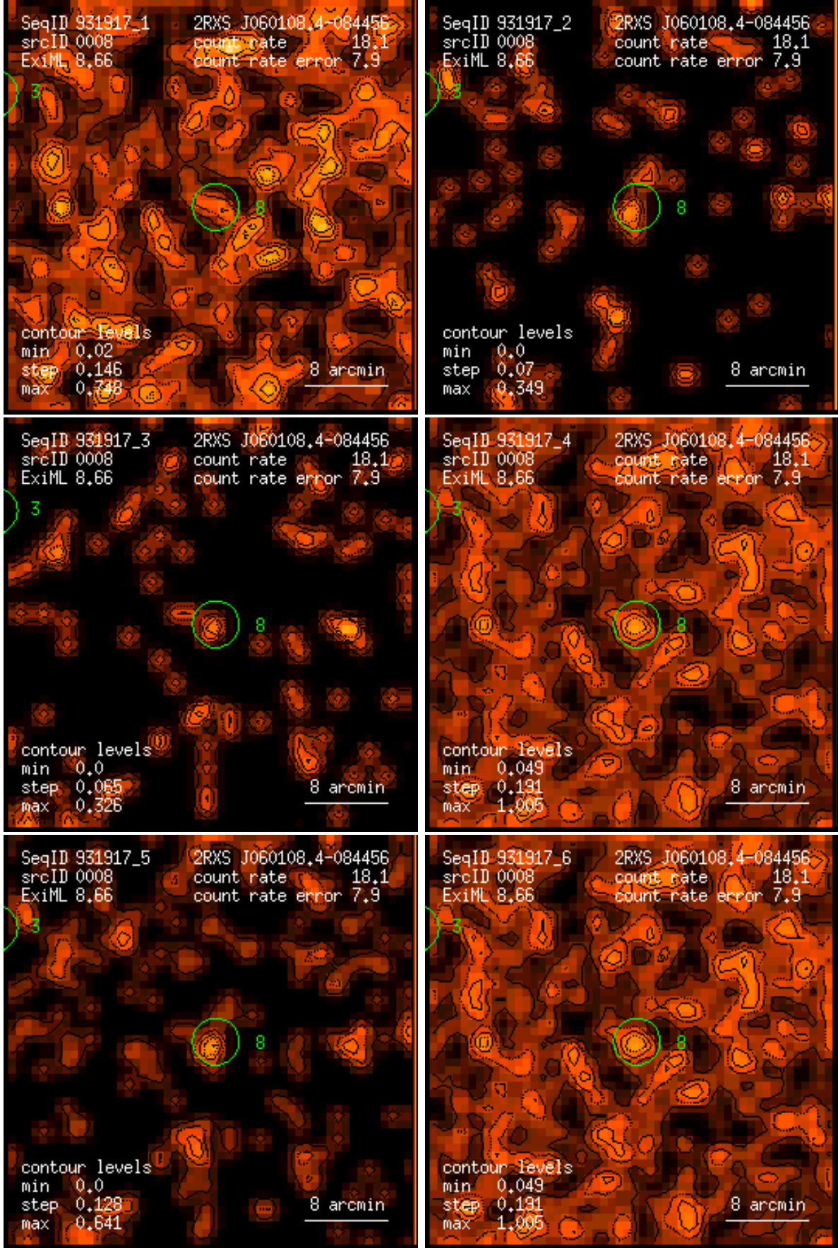
Figure 8: RASS 931917: detection 0008: band rate images, Gaussian filter: (1) PSPC channels 11 – 41, (2) 52 – 90, (3) 91 – 201, (4) 11 – 235, (5) 52 – 201, (6) 11 – 201. Broad band rates in counts/ks. Band rate contour levels in counts/ks/arcmin 2 .
