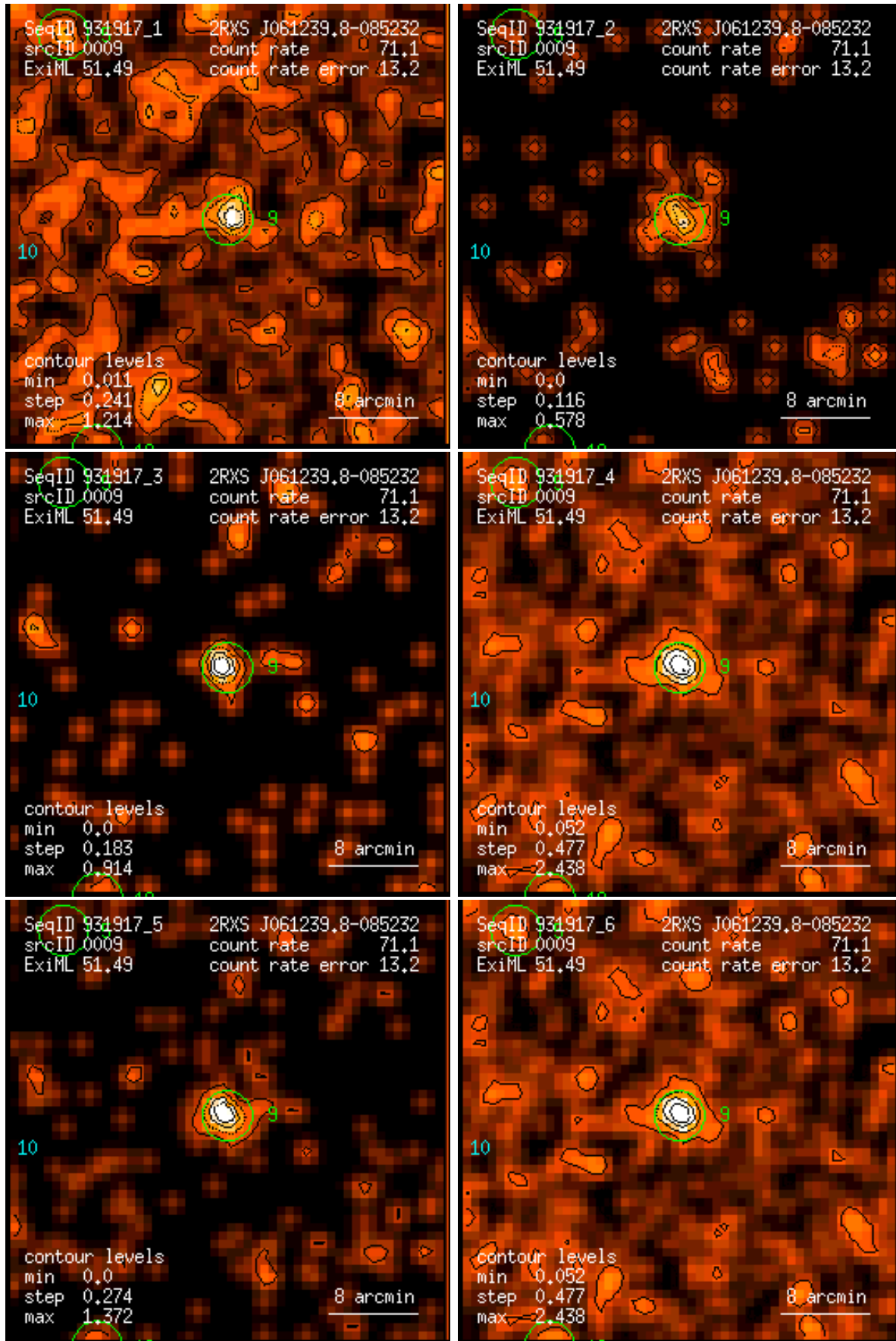
Figure 9: RASS 931917: detection 0009: band rate images, Gaussian filter: (1) PSPC channels 11 – 41, (2) 52 – 90, (3) 91 – 201, (4) 11 – 235, (5) 52 – 201, (6) 11 – 201. Broad band rates in counts/ks. Band rate contour levels in counts/ks/arcmin 2 .
