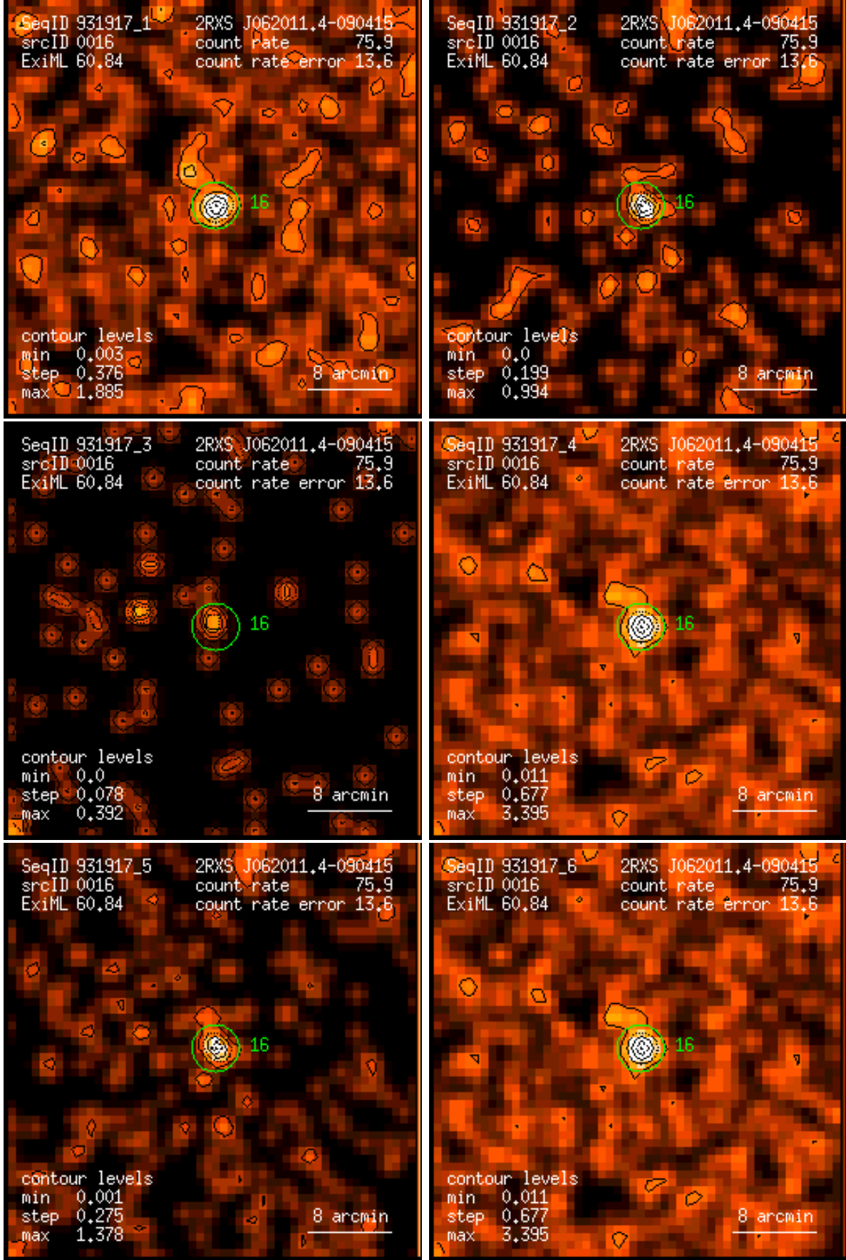
Figure 16: RASS 931917: detection 0016: band rate images, Gaussian filter: (1) PSPC channels 11 – 41, (2) 52 – 90, (3) 91 – 201, (4) 11 – 235, (5) 52 – 201, (6) 11 – 201. Broad band rates in counts/ks. Band rate contour levels in counts/ks/arcmin 2 .
