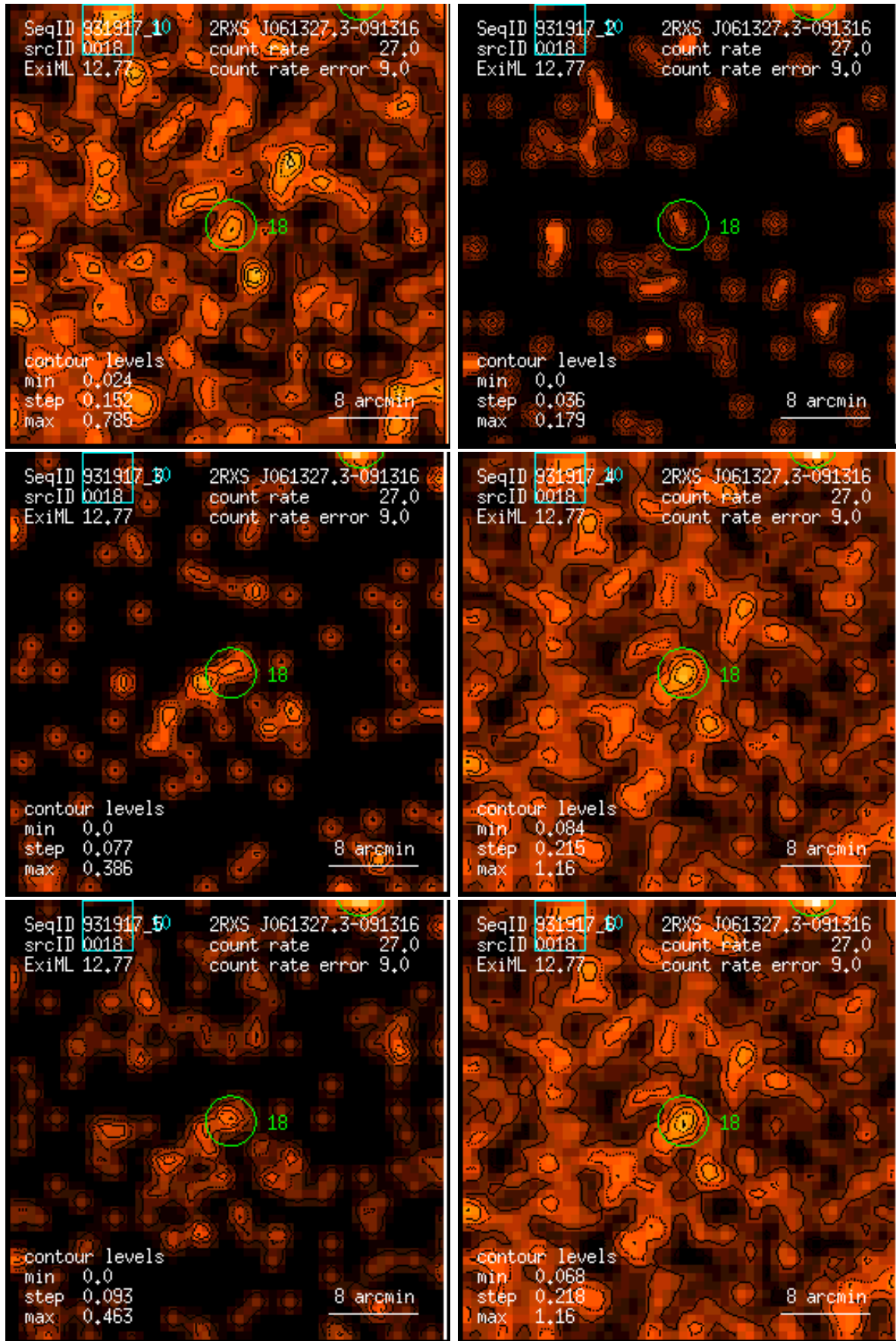
Figure 18: RASS 931917: detection 0018: band rate images, Gaussian filter: (1) PSPC channels 11 – 41, (2) 52 – 90, (3) 91 – 201, (4) 11 – 235, (5) 52 – 201, (6) 11 – 201. Broad band rates in counts/ks. Band rate contour levels in counts/ks/arcmin 2 .
