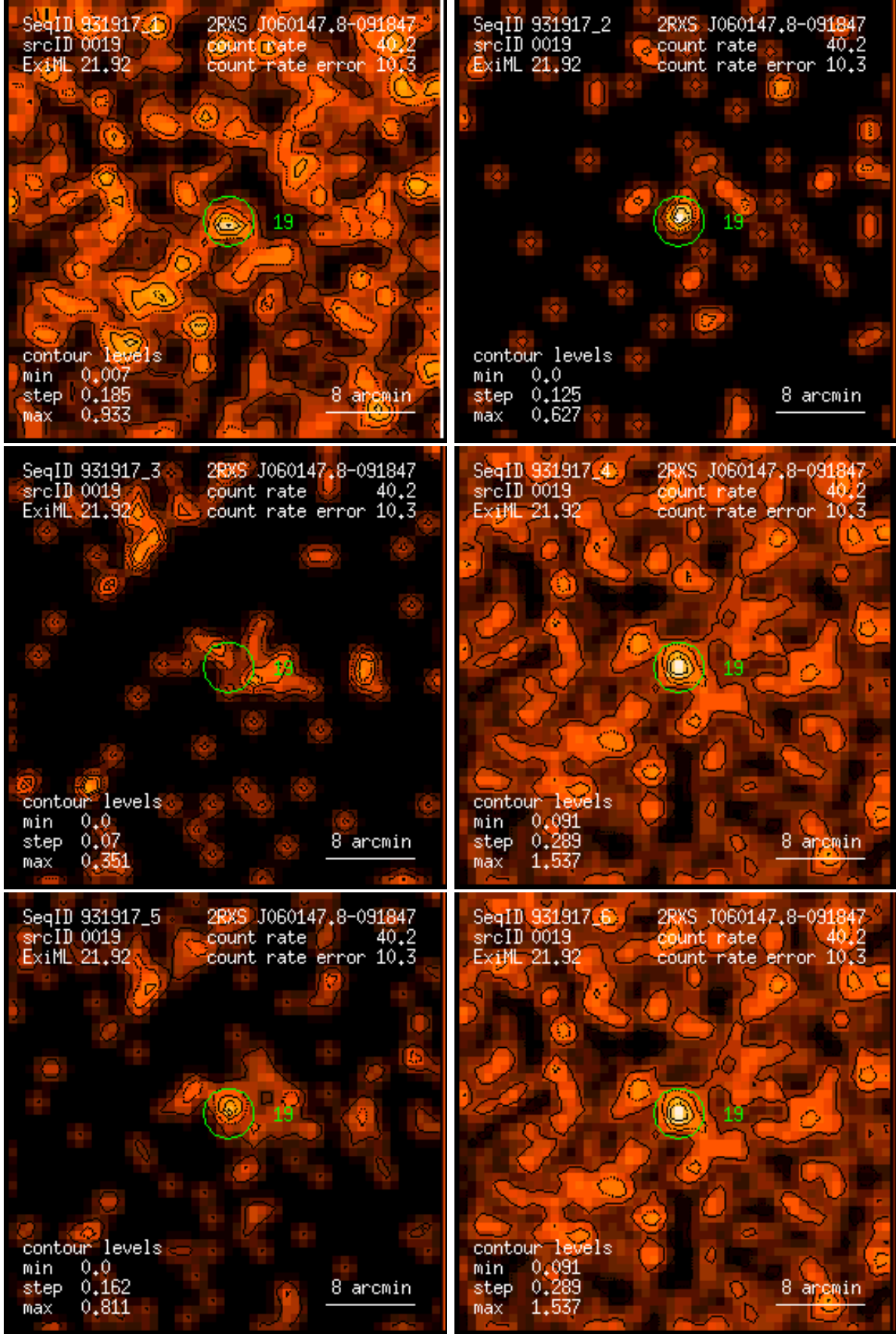
Figure 19: RASS 931917: detection 0019: band rate images, Gaussian filter: (1) PSPC channels 11 – 41, (2) 52 – 90, (3) 91 – 201, (4) 11 – 235, (5) 52 – 201, (6) 11 – 201. Broad band rates in counts/ks. Band rate contour levels in counts/ks/arcmin 2 .
