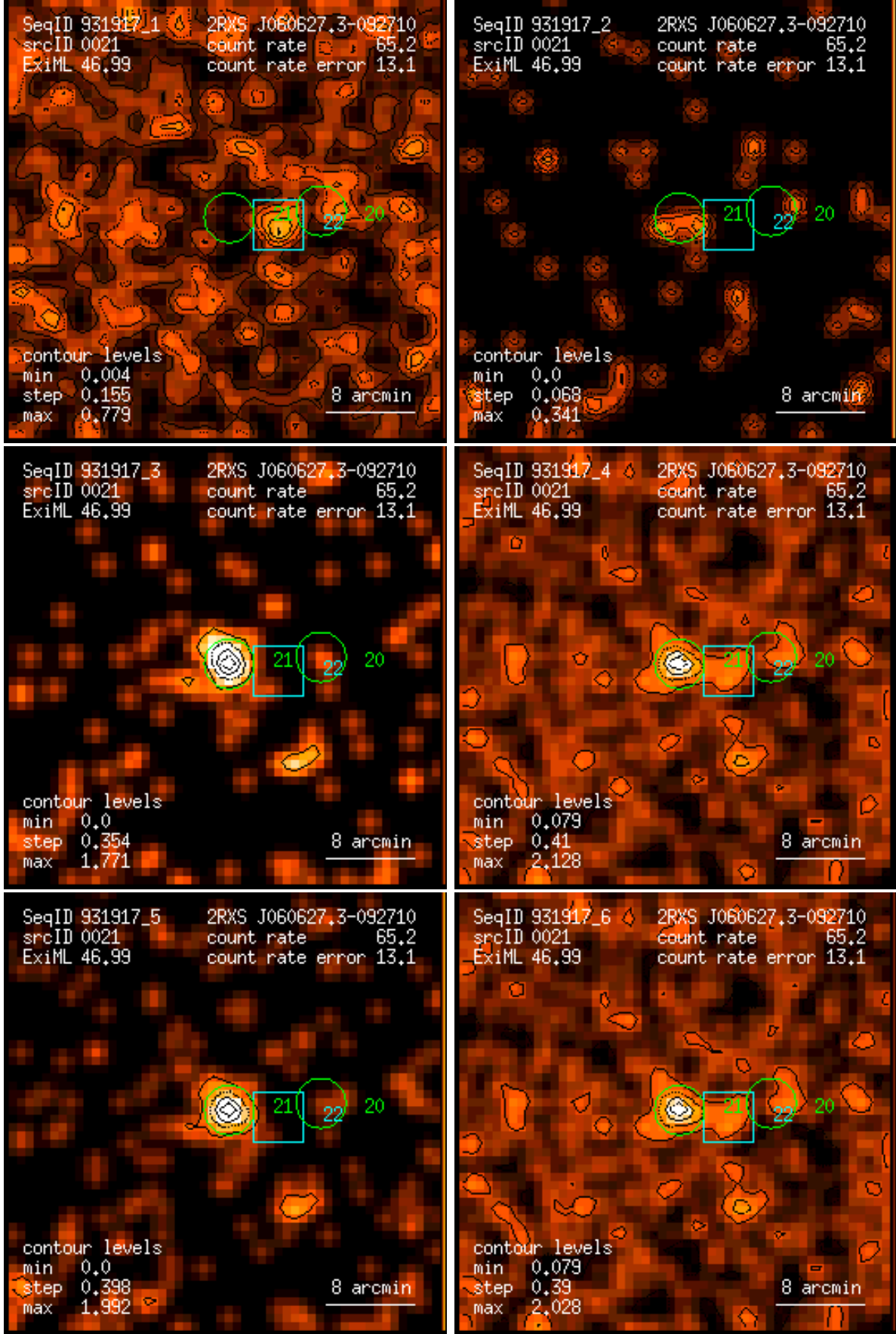
Figure 21: RASS 931917: detection 0021: band rate images, Gaussian filter: (1) PSPC channels 11 – 41, (2) 52 – 90, (3) 91 – 201, (4) 11 – 235, (5) 52 – 201, (6) 11 – 201. Broad band rates in counts/ks. Band rate contour levels in counts/ks/arcmin 2 .
