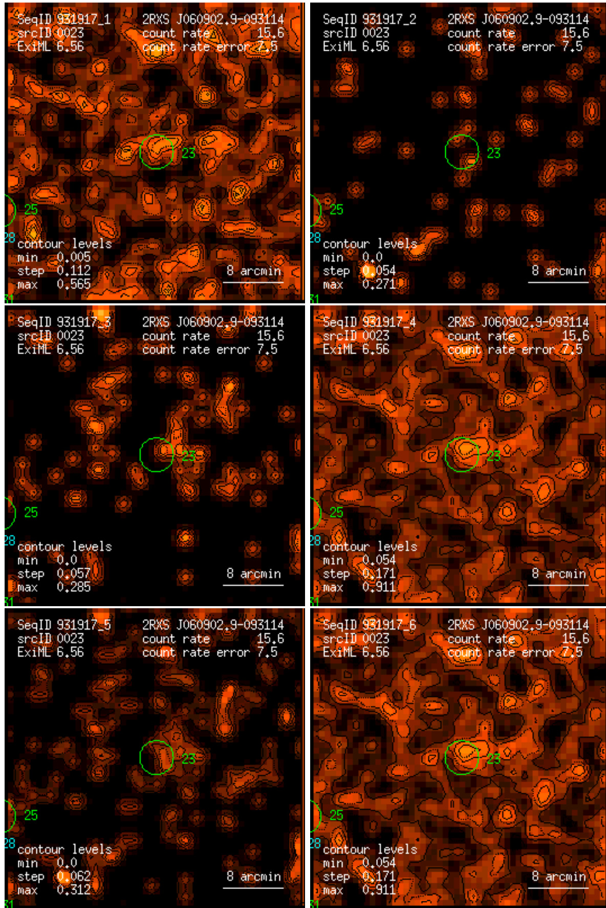
Figure 23: RASS 931917: detection 0023: band rate images, Gaussian filter: (1) PSPC channels 11 – 41, (2) 52 – 90, (3) 91 – 201, (4) 11 – 235, (5) 52 – 201, (6) 11 – 201. Broad band rates in counts/ks. Band rate contour levels in counts/ks/arcmin 2 .
