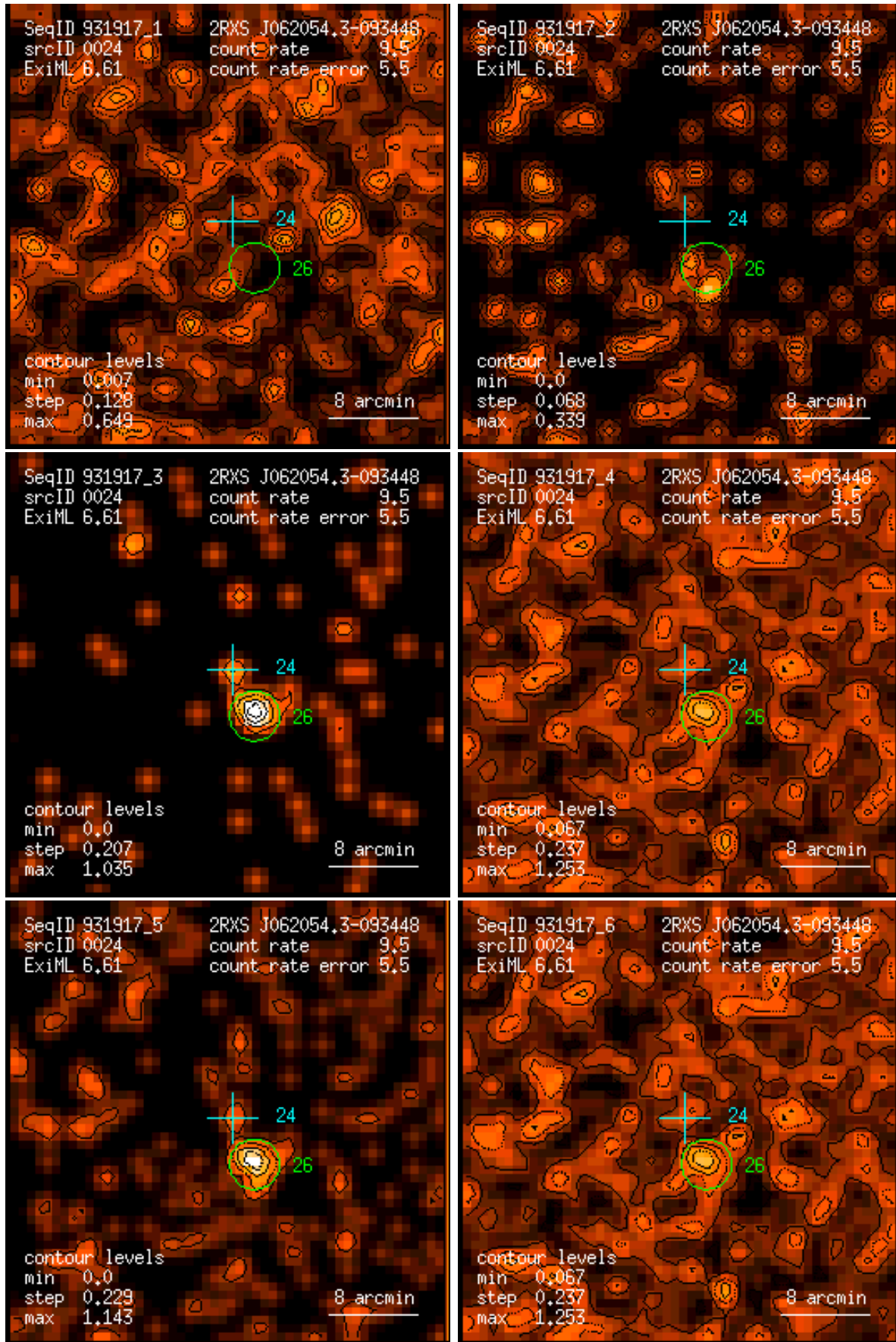
Figure 24: RASS 931917: detection 0024: band rate images, Gaussian filter: (1) PSPC channels 11 – 41, (2) 52 – 90, (3) 91 – 201, (4) 11 – 235, (5) 52 – 201, (6) 11 – 201. Broad band rates in counts/ks. Band rate contour levels in counts/ks/arcmin 2 .
