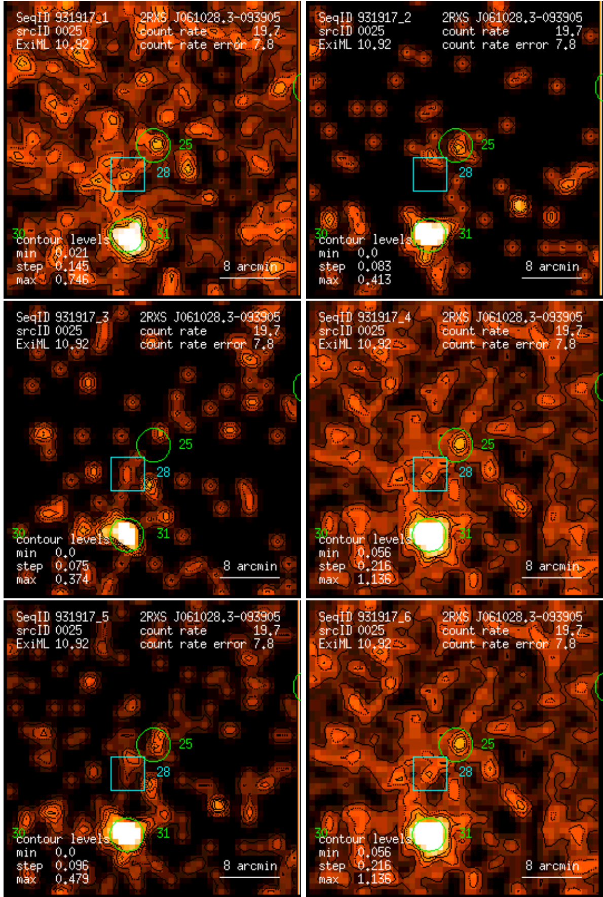
Figure 25: RASS 931917: detection 0025: band rate images, Gaussian filter: (1) PSPC channels 11 – 41, (2) 52 – 90, (3) 91 – 201, (4) 11 – 235, (5) 52 – 201, (6) 11 – 201. Broad band rates in counts/ks. Band rate contour levels in counts/ks/arcmin 2 .
