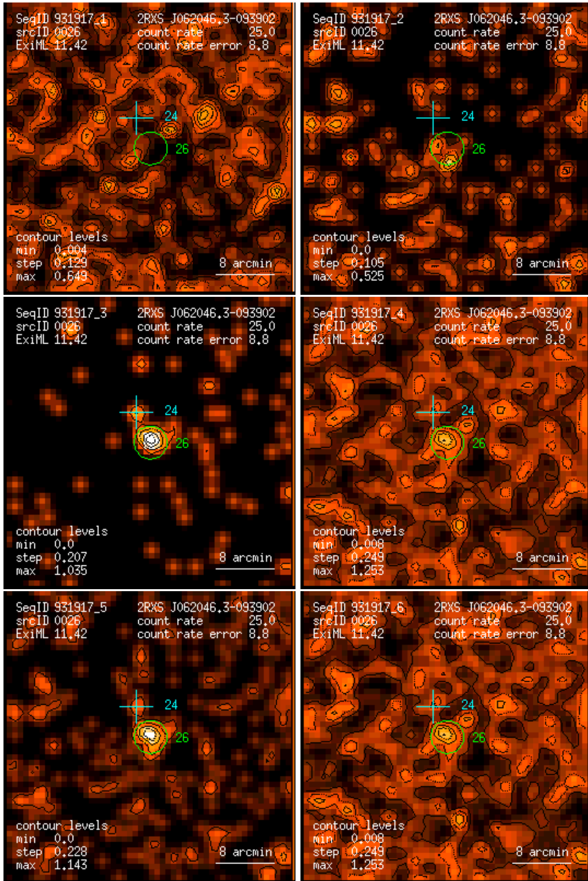
Figure 26: RASS 931917: detection 0026: band rate images, Gaussian filter: (1) PSPC channels 11 – 41, (2) 52 – 90, (3) 91 – 201, (4) 11 – 235, (5) 52 – 201, (6) 11 – 201. Broad band rates in counts/ks. Band rate contour levels in counts/ks/arcmin 2 .
