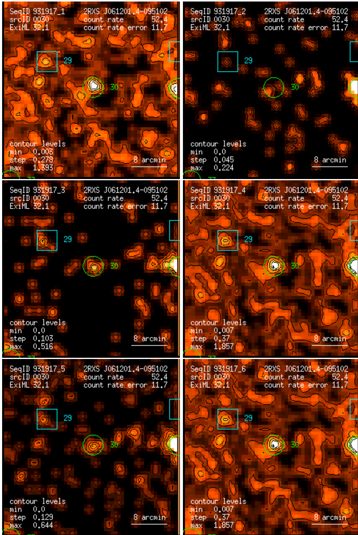
Figure 30: RASS 931917: detection 0030: band rate images, Gaussian filter: (1) PSPC channels 11 – 41, (2) 52 – 90, (3) 91 – 201, (4) 11 – 235, (5) 52 – 201, (6) 11 – 201. Broad band rates in counts/ks. Band rate contour levels in counts/ks/arcmin 2 .
