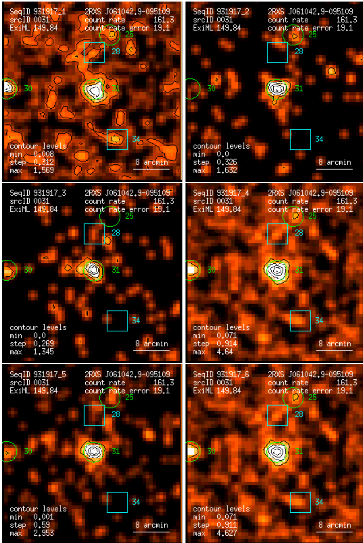
Figure 31: RASS 931917: detection 0031: band rate images, Gaussian filter: (1) PSPC channels 11 – 41, (2) 52 – 90, (3) 91 – 201, (4) 11 – 235, (5) 52 – 201, (6) 11 – 201. Broad band rates in counts/ks. Band rate contour levels in counts/ks/arcmin 2 .
