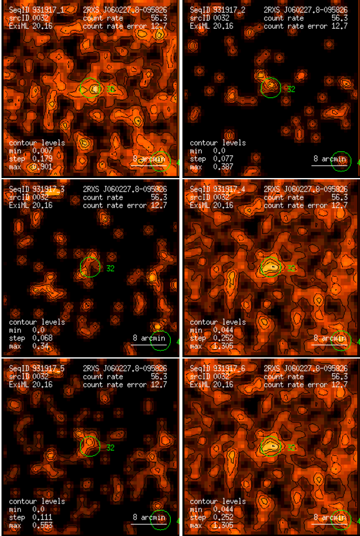
Figure 32: RASS 931917: detection 0032: band rate images, Gaussian filter: (1) PSPC channels 11 – 41, (2) 52 – 90, (3) 91 – 201, (4) 11 – 235, (5) 52 – 201, (6) 11 – 201. Broad band rates in counts/ks. Band rate contour levels in counts/ks/arcmin 2 .
