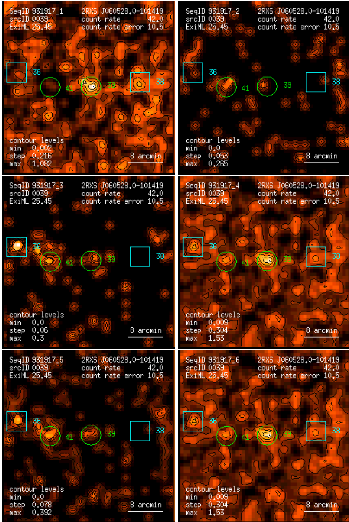
Figure 39: RASS 931917: detection 0039: band rate images, Gaussian filter: (1) PSPC channels 11 – 41, (2) 52 – 90, (3) 91 – 201, (4) 11 – 235, (5) 52 – 201, (6) 11 – 201. Broad band rates in counts/ks. Band rate contour levels in counts/ks/arcmin 2 .
