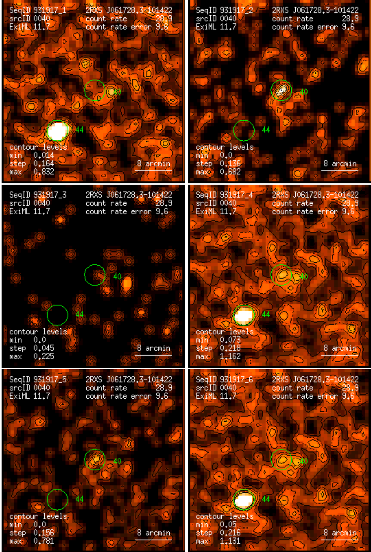
Figure 40: RASS 931917: detection 0040: band rate images, Gaussian filter: (1) PSPC channels 11 – 41, (2) 52 – 90, (3) 91 – 201, (4) 11 – 235, (5) 52 – 201, (6) 11 – 201. Broad band rates in counts/ks. Band rate contour levels in counts/ks/arcmin 2 .
