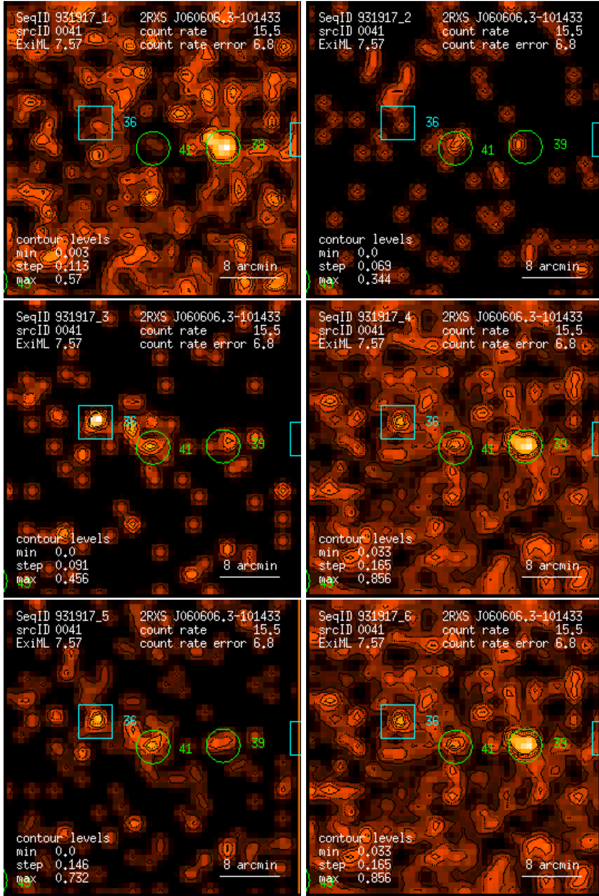
Figure 41: RASS 931917: detection 0041: band rate images, Gaussian filter: (1) PSPC channels 11 – 41, (2) 52 – 90, (3) 91 – 201, (4) 11 – 235, (5) 52 – 201, (6) 11 – 201. Broad band rates in counts/ks. Band rate contour levels in counts/ks/arcmin 2 .
