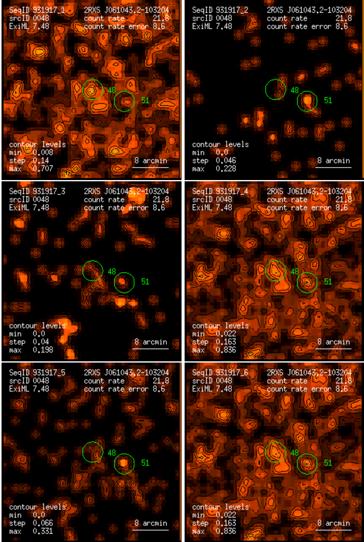
Figure 48: RASS 931917: detection 0048: band rate images, Gaussian filter: (1) PSPC channels 11 – 41, (2) 52 – 90, (3) 91 – 201, (4) 11 – 235, (5) 52 – 201, (6) 11 – 201. Broad band rates in counts/ks. Band rate contour levels in counts/ks/arcmin 2 .
