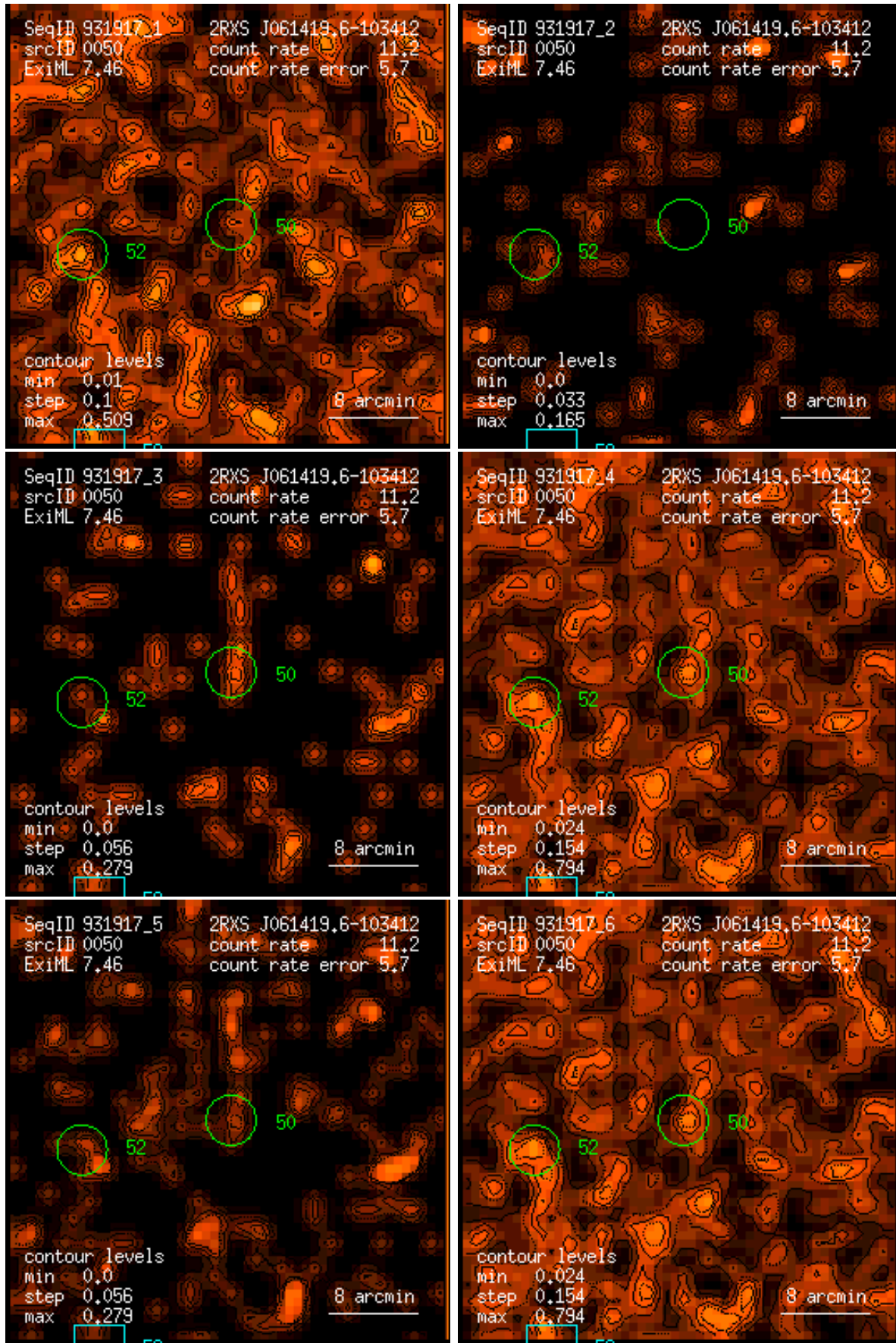
Figure 50: RASS 931917: detection 0050: band rate images, Gaussian filter: (1) PSPC channels 11 – 41, (2) 52 – 90, (3) 91 – 201, (4) 11 – 235, (5) 52 – 201, (6) 11 – 201. Broad band rates in counts/ks. Band rate contour levels in counts/ks/arcmin 2 .
