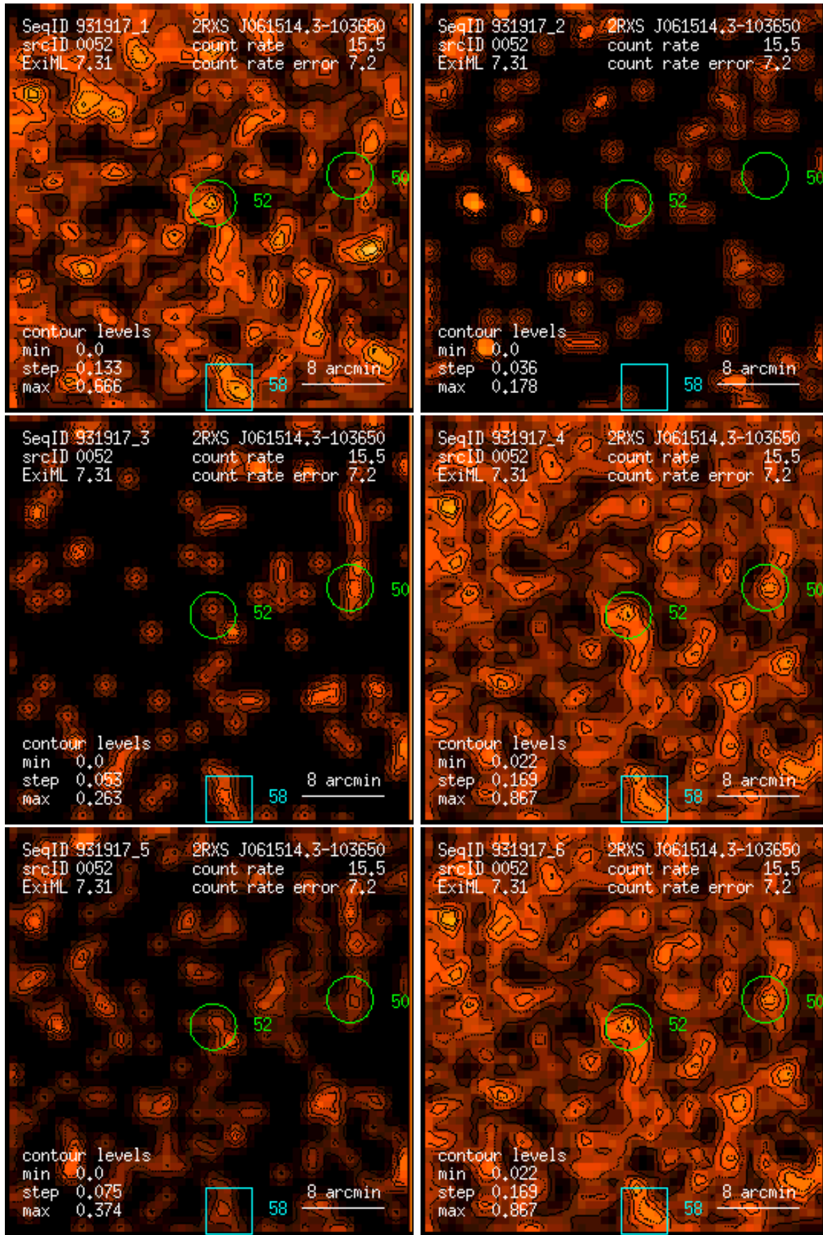
Figure 52: RASS 931917: detection 0052: band rate images, Gaussian filter: (1) PSPC channels 11 – 41, (2) 52 – 90, (3) 91 – 201, (4) 11 – 235, (5) 52 – 201, (6) 11 – 201. Broad band rates in counts/ks. Band rate contour levels in counts/ks/arcmin 2 .
