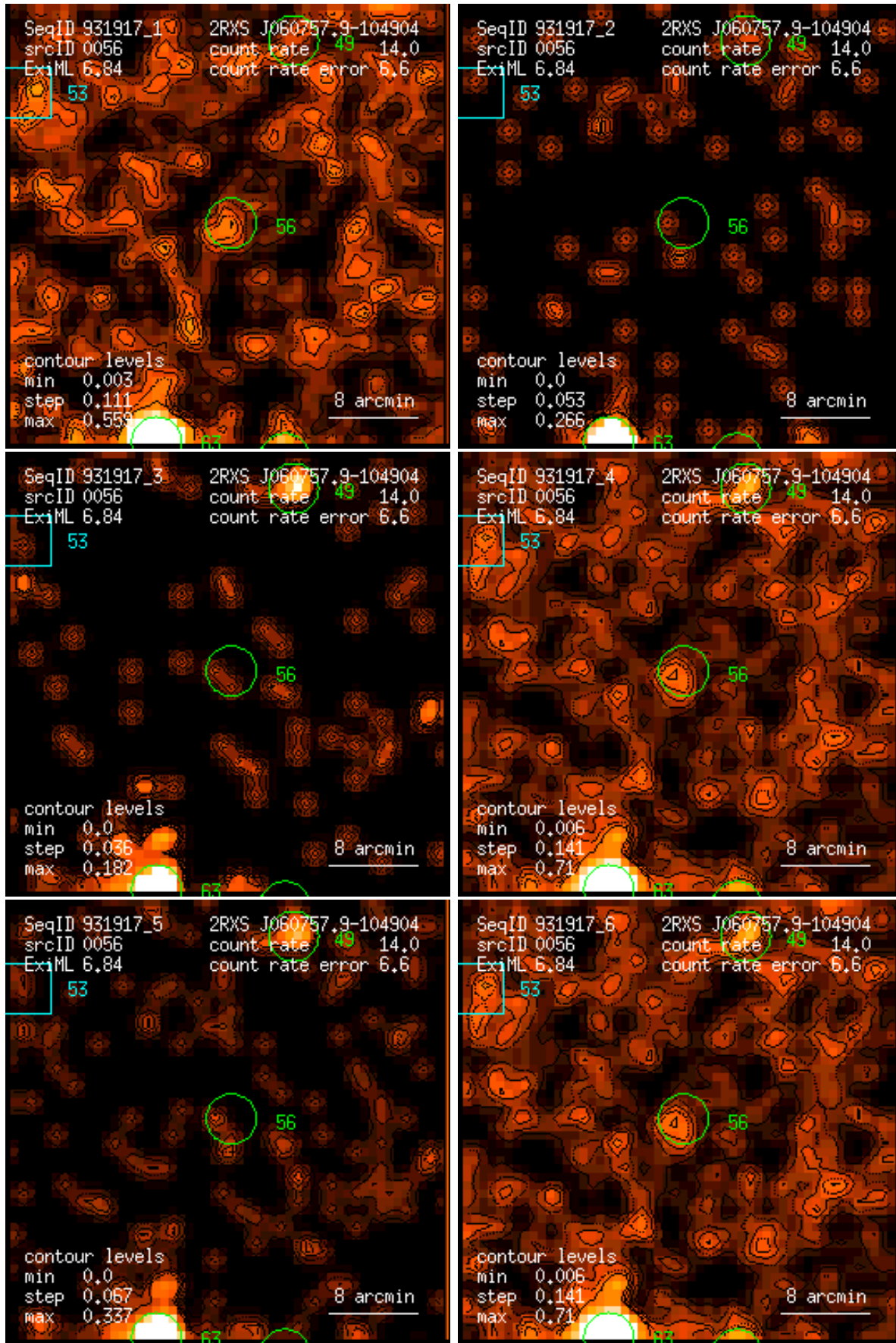
Figure 56: RASS 931917: detection 0056: band rate images, Gaussian filter: (1) PSPC channels 11 – 41, (2) 52 – 90, (3) 91 – 201, (4) 11 – 235, (5) 52 – 201, (6) 11 – 201. Broad band rates in counts/ks. Band rate contour levels in counts/ks/arcmin 2 .
