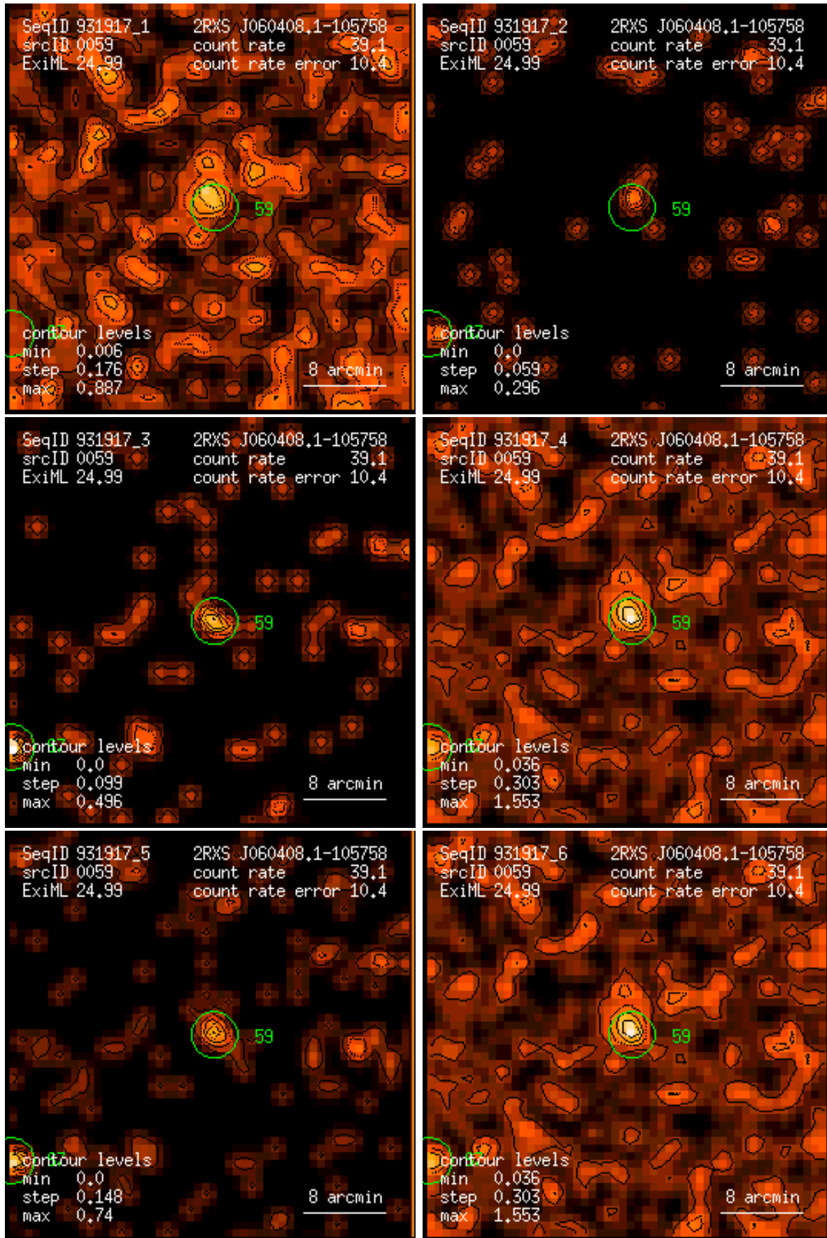
Figure 59: RASS 931917: detection 0059: band rate images, Gaussian filter: (1) PSPC channels 11 – 41, (2) 52 – 90, (3) 91 – 201, (4) 11 – 235, (5) 52 – 201, (6) 11 – 201. Broad band rates in counts/ks. Band rate contour levels in counts/ks/arcmin 2 .
