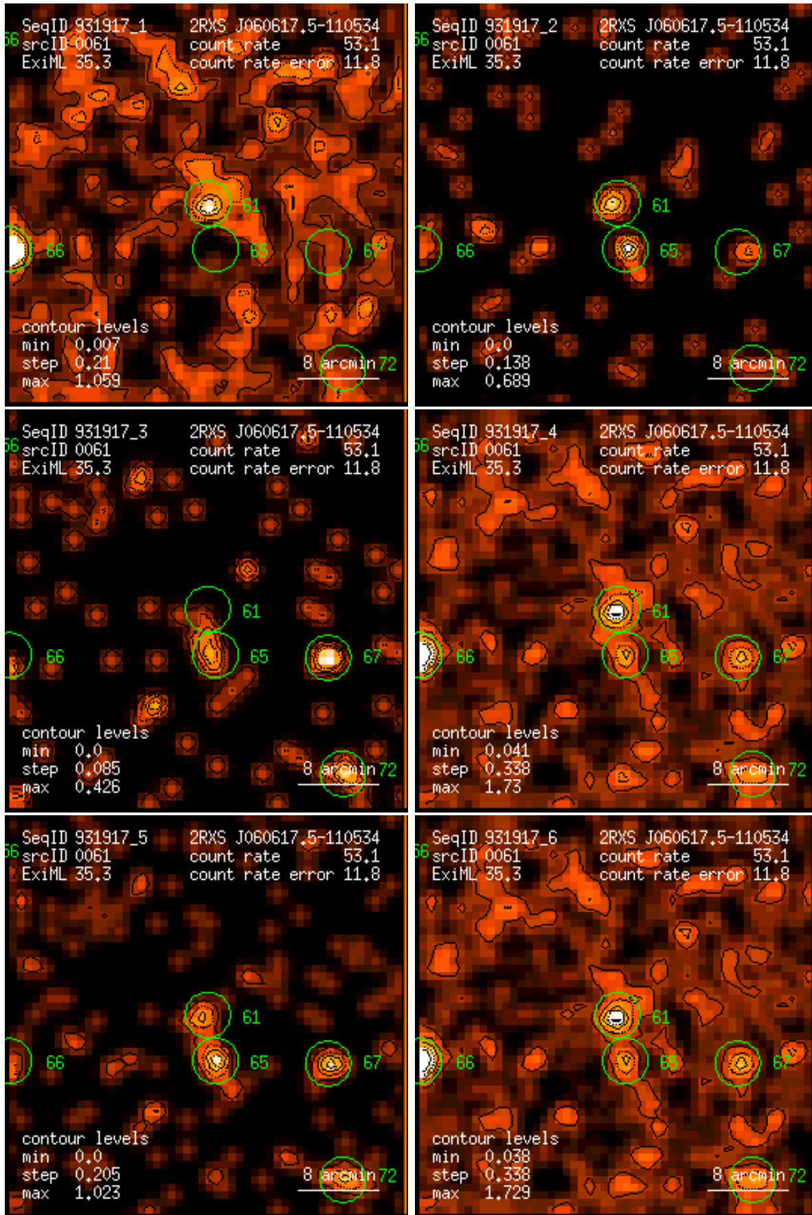
Figure 61: RASS 931917: detection 0061: band rate images, Gaussian filter: (1) PSPC channels 11 – 41, (2) 52 – 90, (3) 91 – 201, (4) 11 – 235, (5) 52 – 201, (6) 11 – 201. Broad band rates in counts/ks. Band rate contour levels in counts/ks/arcmin 2 .
