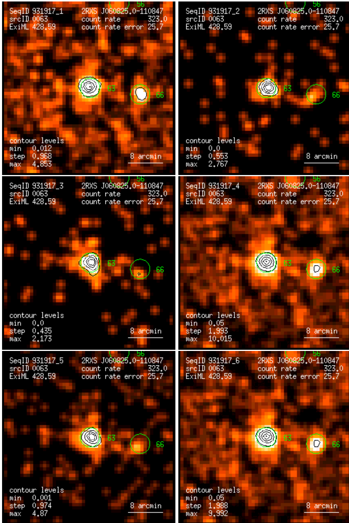
Figure 63: RASS 931917: detection 0063: band rate images, Gaussian filter: (1) PSPC channels 11 – 41, (2) 52 – 90, (3) 91 – 201, (4) 11 – 235, (5) 52 – 201, (6) 11 – 201. Broad band rates in counts/ks. Band rate contour levels in counts/ks/arcmin 2 .
