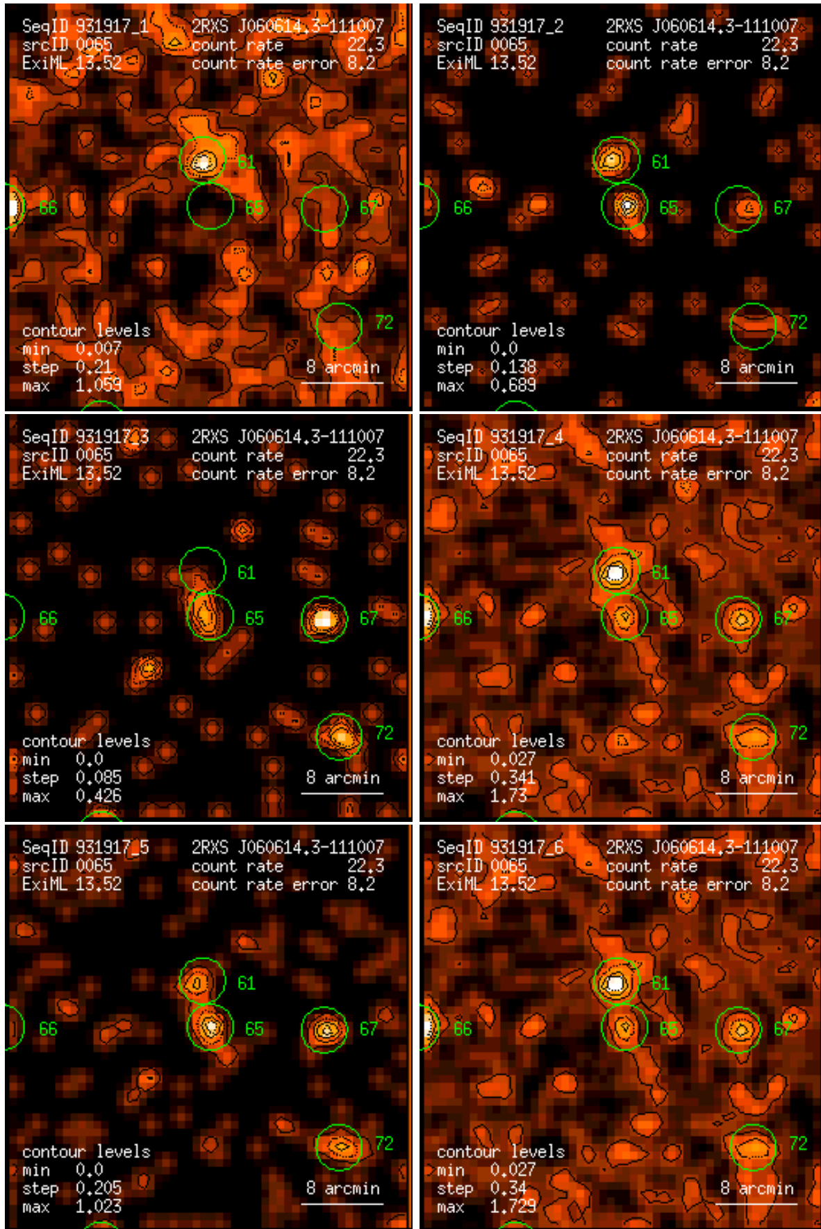
Figure 65: RASS 931917: detection 0065: band rate images, Gaussian filter: (1) PSPC channels 11 – 41, (2) 52 – 90, (3) 91 – 201, (4) 11 – 235, (5) 52 – 201, (6) 11 – 201. Broad band rates in counts/ks. Band rate contour levels in counts/ks/arcmin 2 .
