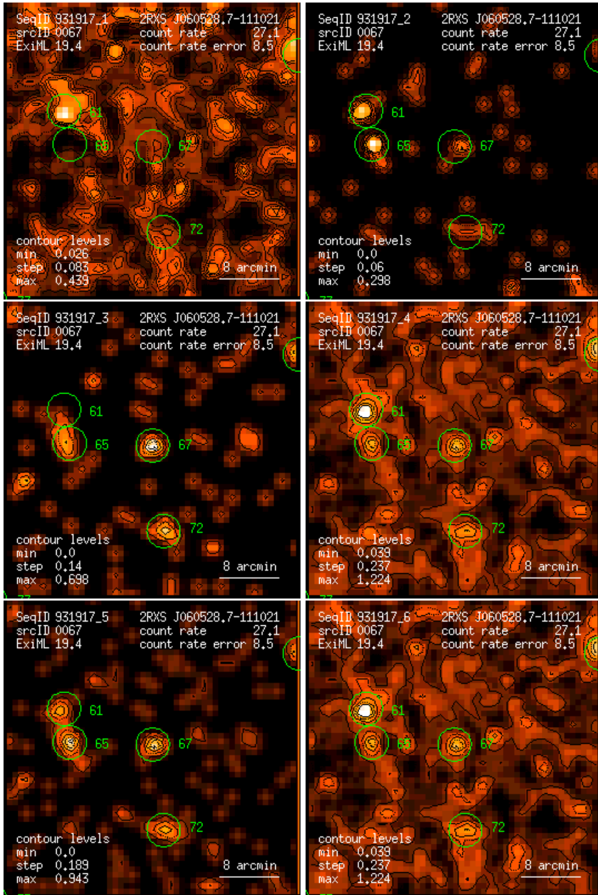
Figure 67: RASS 931917: detection 0067: band rate images, Gaussian filter: (1) PSPC channels 11 – 41, (2) 52 – 90, (3) 91 – 201, (4) 11 – 235, (5) 52 – 201, (6) 11 – 201. Broad band rates in counts/ks. Band rate contour levels in counts/ks/arcmin 2 .
