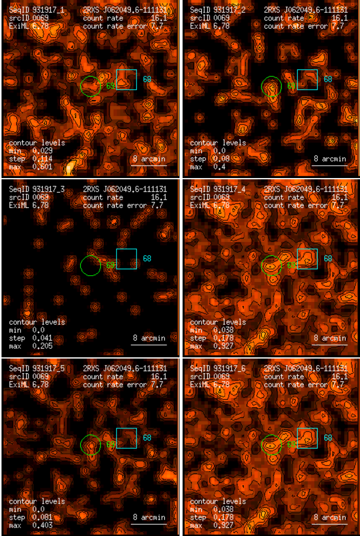
Figure 69: RASS 931917: detection 0069: band rate images, Gaussian filter: (1) PSPC channels 11 – 41, (2) 52 – 90, (3) 91 – 201, (4) 11 – 235, (5) 52 – 201, (6) 11 – 201. Broad band rates in counts/ks. Band rate contour levels in counts/ks/arcmin 2 .
