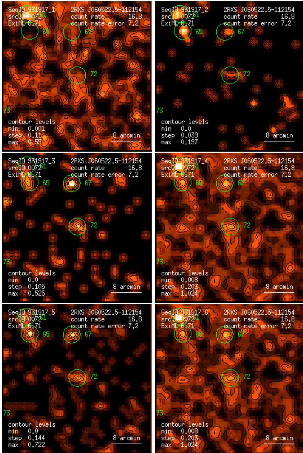
Figure 72: RASS 931917: detection 0072: band rate images, Gaussian filter: (1) PSPC channels 11 – 41, (2) 52 – 90, (3) 91 – 201, (4) 11 – 235, (5) 52 – 201, (6) 11 – 201. Broad band rates in counts/ks. Band rate contour levels in counts/ks/arcmin 2 .
