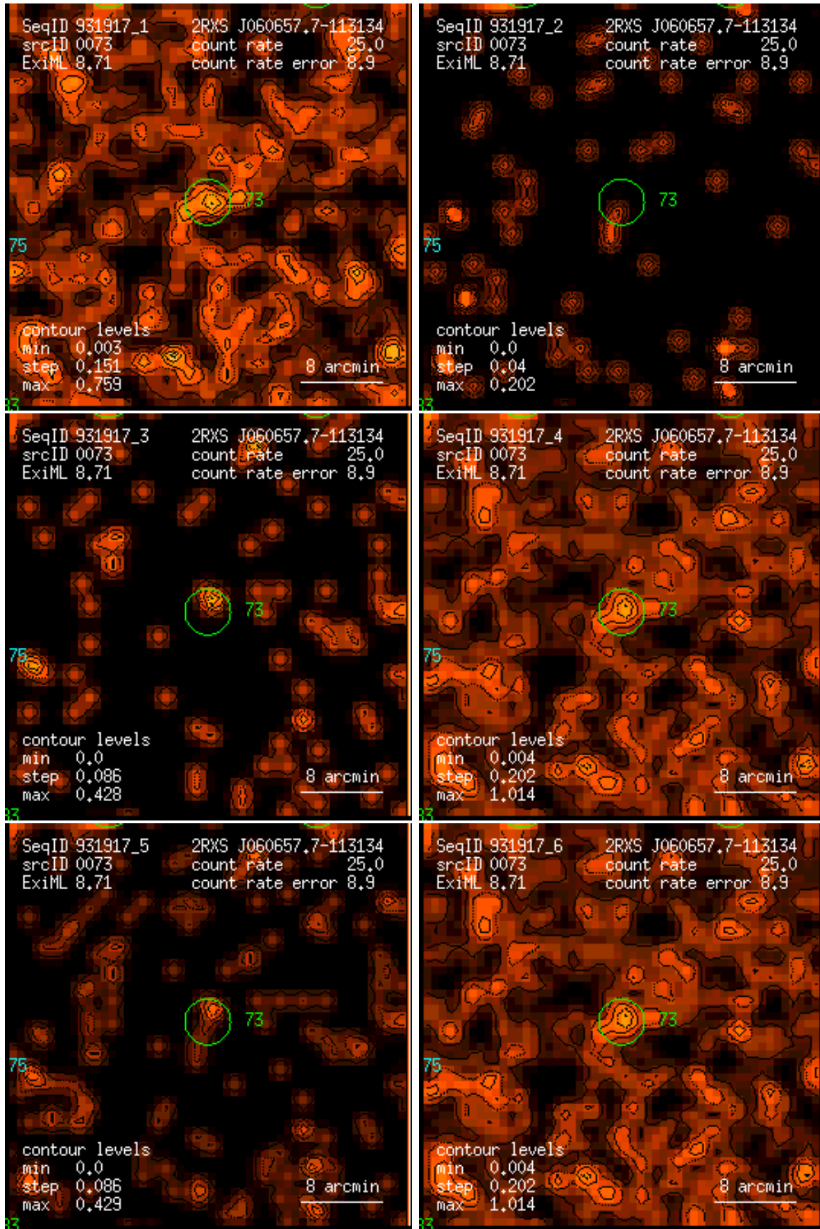
Figure 73: RASS 931917: detection 0073: band rate images, Gaussian filter: (1) PSPC channels 11 – 41, (2) 52 – 90, (3) 91 – 201, (4) 11 – 235, (5) 52 – 201, (6) 11 – 201. Broad band rates in counts/ks. Band rate contour levels in counts/ks/arcmin 2 .
