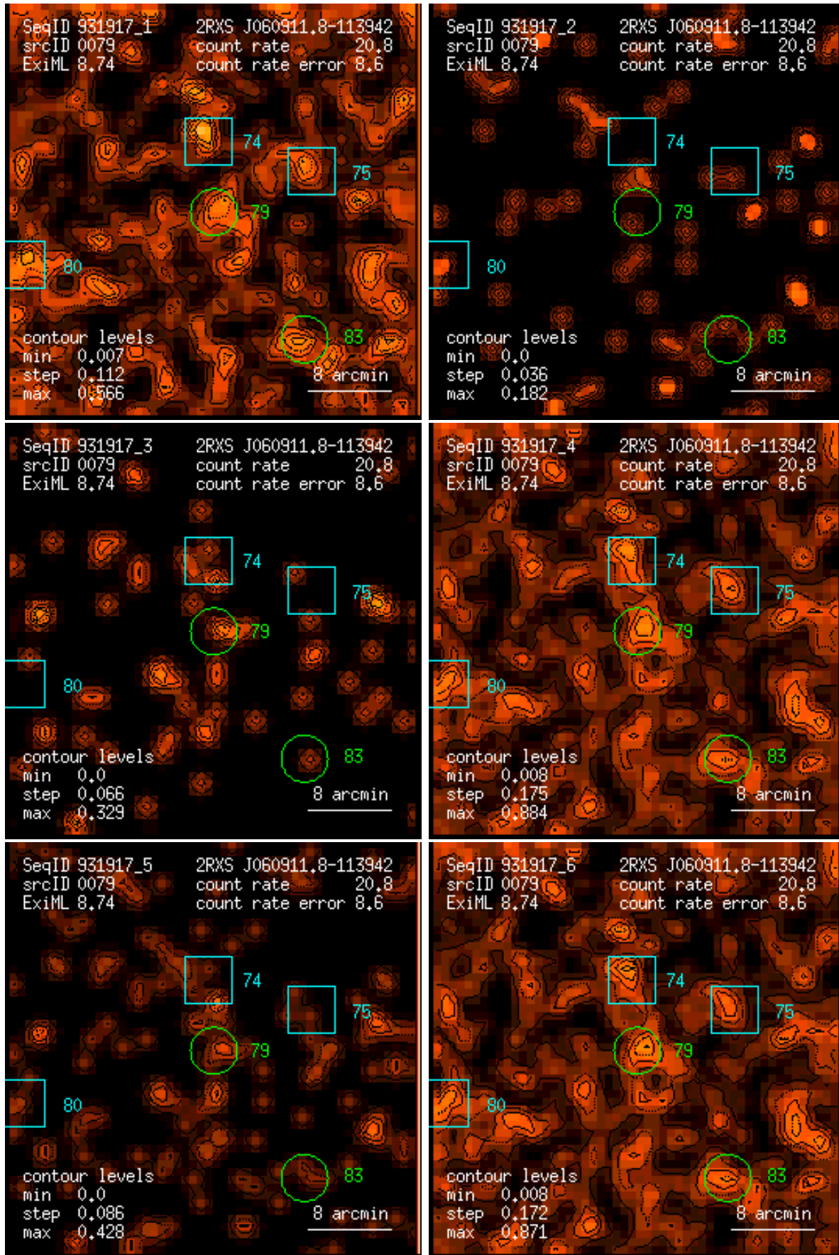
Figure 79: RASS 931917: detection 0079: band rate images, Gaussian filter: (1) PSPC channels 11 – 41, (2) 52 – 90, (3) 91 – 201, (4) 11 – 235, (5) 52 – 201, (6) 11 – 201. Broad band rates in counts/ks. Band rate contour levels in counts/ks/arcmin 2 .
