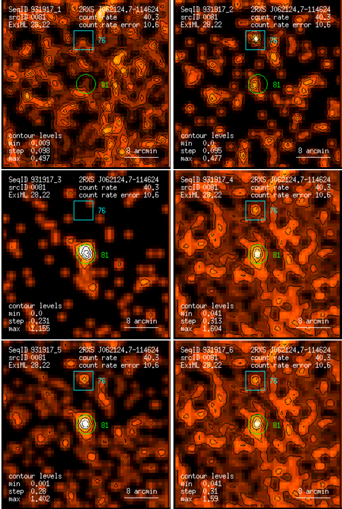
Figure 81: RASS 931917: detection 0081: band rate images, Gaussian filter: (1) PSPC channels 11 – 41, (2) 52 – 90, (3) 91 – 201, (4) 11 – 235, (5) 52 – 201, (6) 11 – 201. Broad band rates in counts/ks. Band rate contour levels in counts/ks/arcmin 2 .
