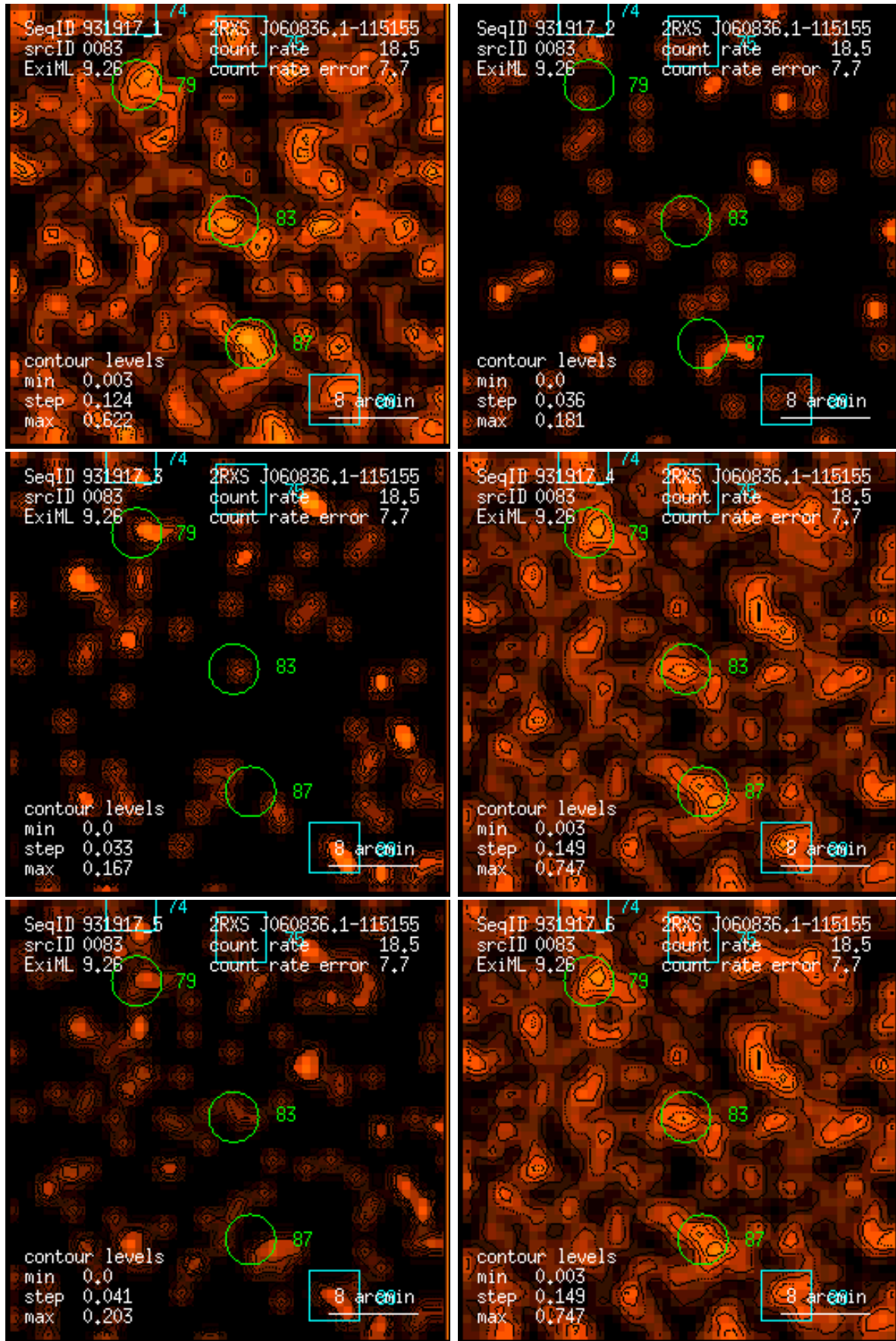
Figure 83: RASS 931917: detection 0083: band rate images, Gaussian filter: (1) PSPC channels 11 – 41, (2) 52 – 90, (3) 91 – 201, (4) 11 – 235, (5) 52 – 201, (6) 11 – 201. Broad band rates in counts/ks. Band rate contour levels in counts/ks/arcmin 2 .
