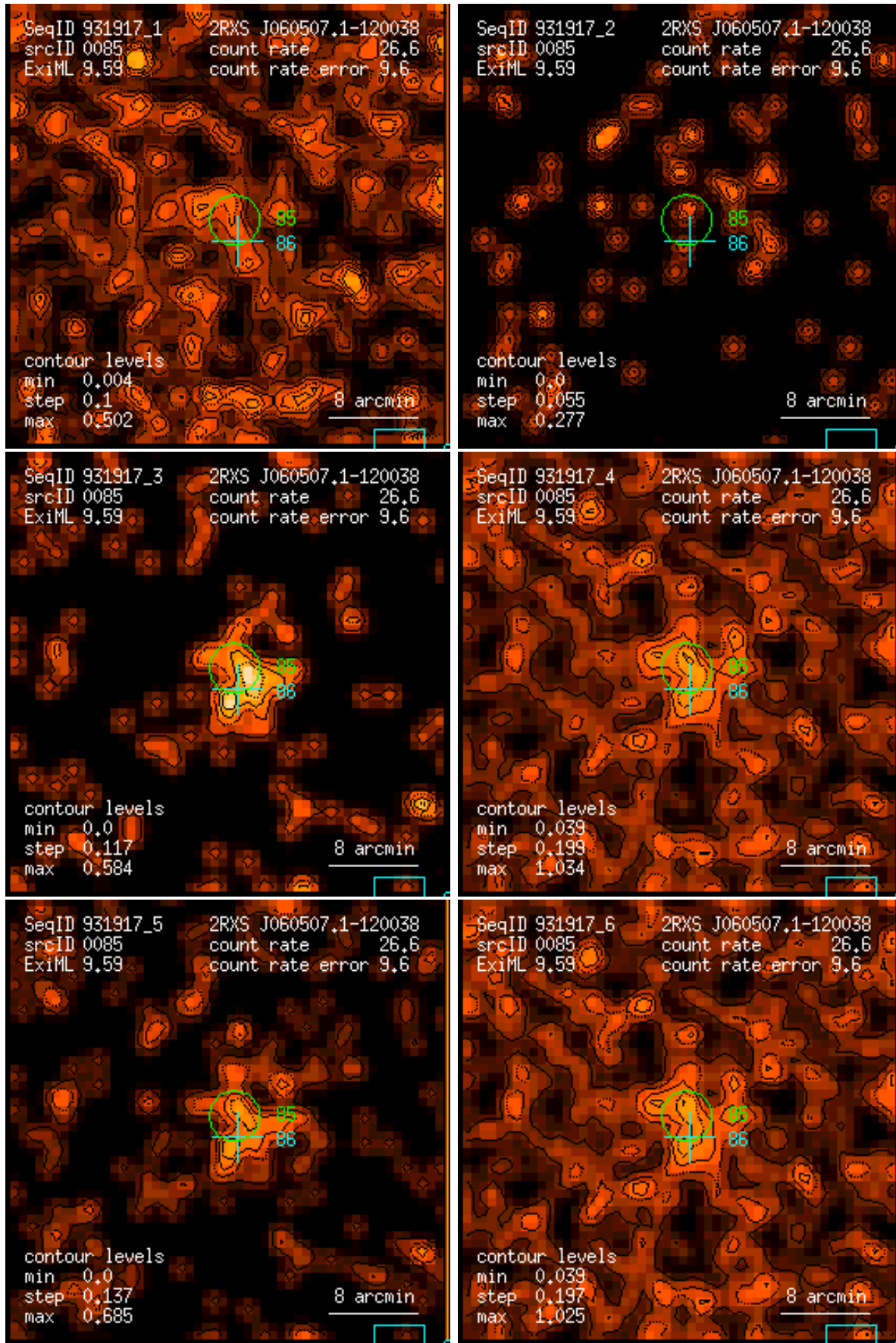
Figure 85: RASS 931917: detection 0085: band rate images, Gaussian filter: (1) PSPC channels 11 – 41, (2) 52 – 90, (3) 91 – 201, (4) 11 – 235, (5) 52 – 201, (6) 11 – 201. Broad band rates in counts/ks. Band rate contour levels in counts/ks/arcmin 2 .
