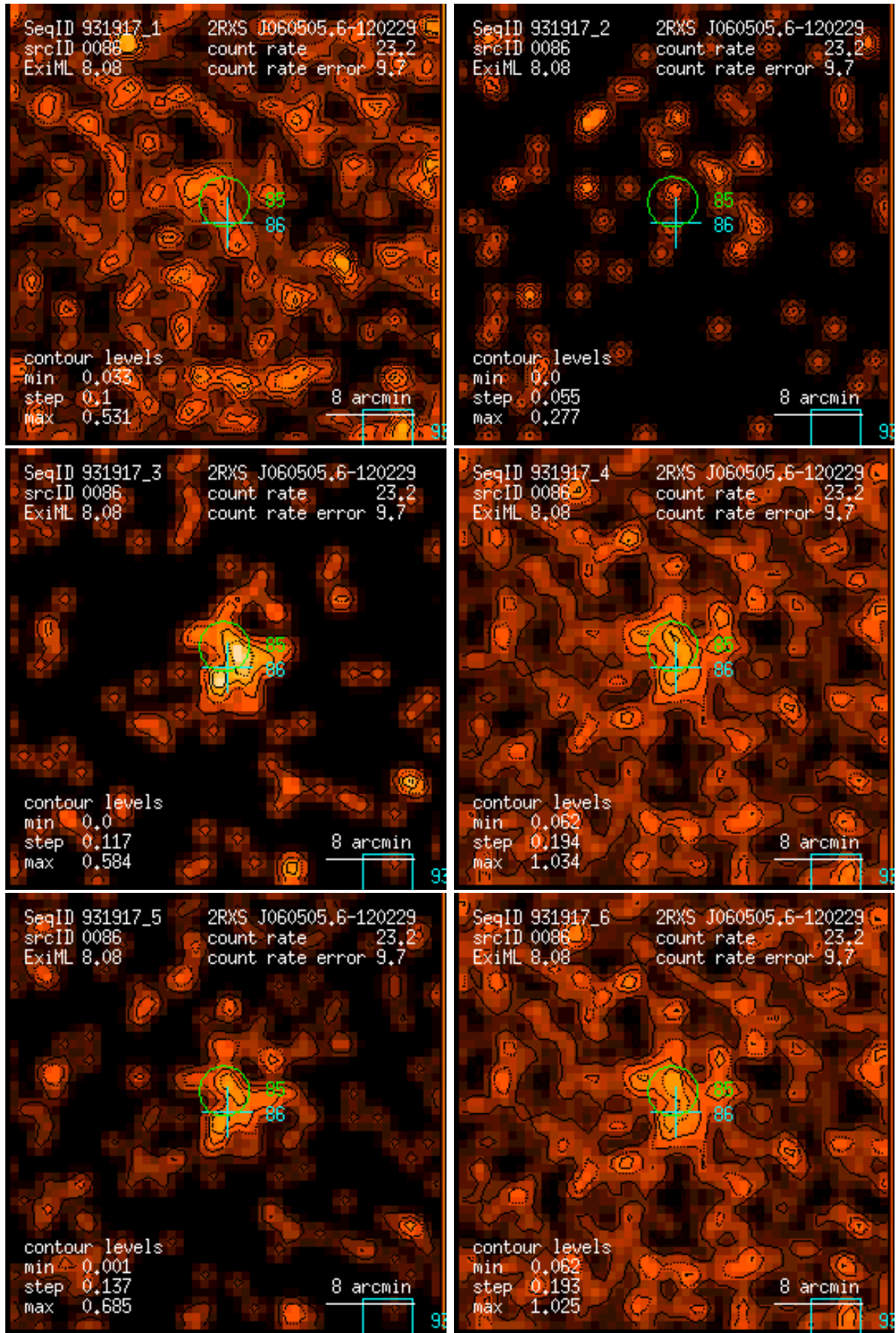
Figure 86: RASS 931917: detection 0086: band rate images, Gaussian filter: (1) PSPC channels 11 – 41, (2) 52 – 90, (3) 91 – 201, (4) 11 – 235, (5) 52 – 201, (6) 11 – 201. Broad band rates in counts/ks. Band rate contour levels in counts/ks/arcmin 2 .
