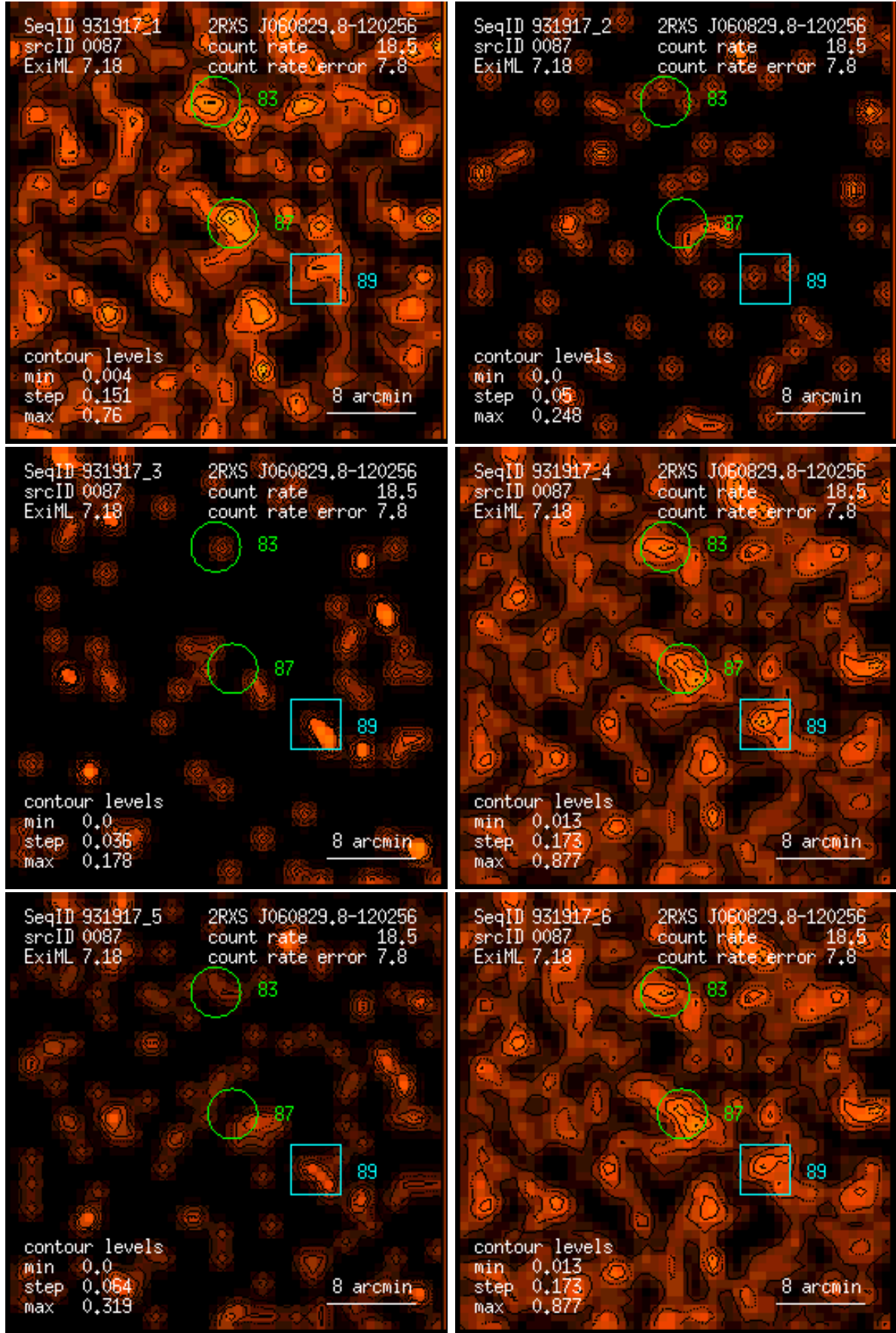
Figure 87: RASS 931917: detection 0087: band rate images, Gaussian filter: (1) PSPC channels 11 – 41, (2) 52 – 90, (3) 91 – 201, (4) 11 – 235, (5) 52 – 201, (6) 11 – 201. Broad band rates in counts/ks. Band rate contour levels in counts/ks/arcmin 2 .
