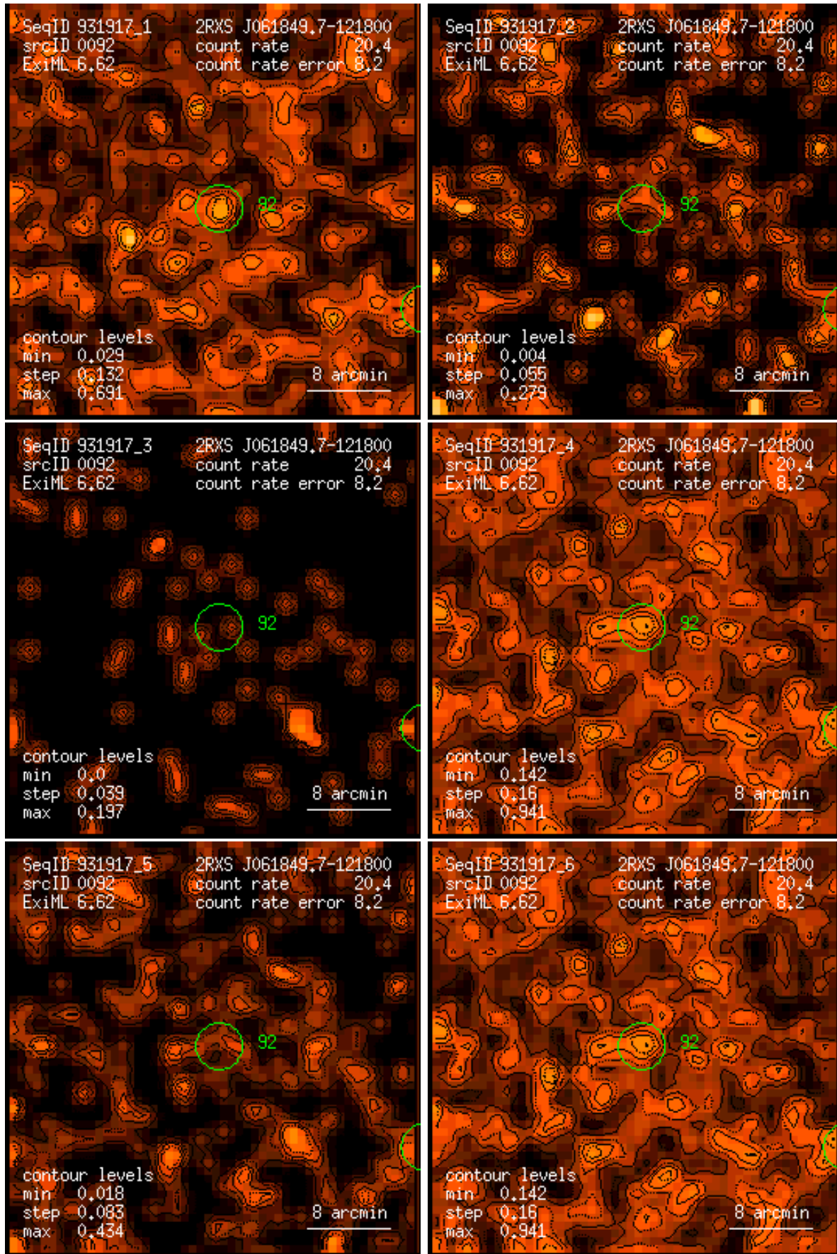
Figure 92: RASS 931917: detection 0092: band rate images, Gaussian filter: (1) PSPC channels 11 – 41, (2) 52 – 90, (3) 91 – 201, (4) 11 – 235, (5) 52 – 201, (6) 11 – 201. Broad band rates in counts/ks. Band rate contour levels in counts/ks/arcmin 2 .
