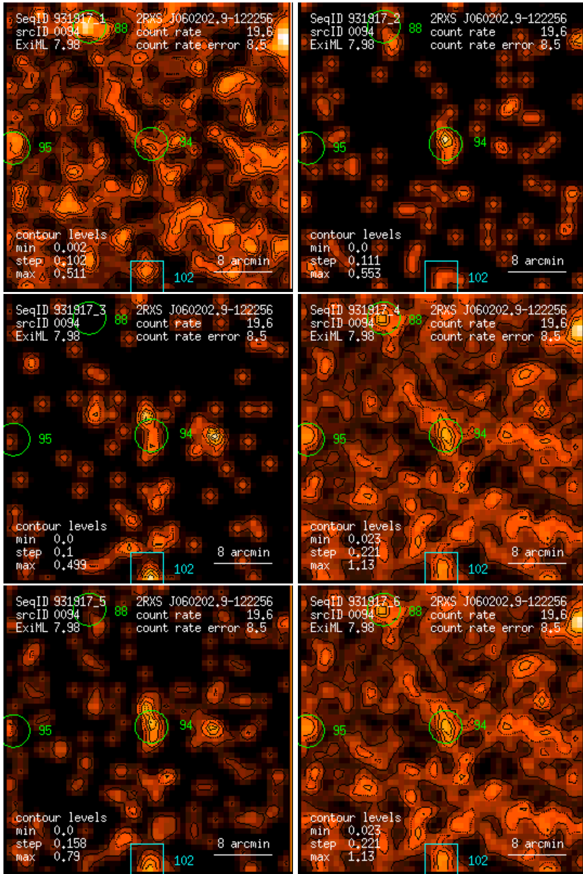
Figure 94: RASS 931917: detection 0094: band rate images, Gaussian filter: (1) PSPC channels 11 – 41, (2) 52 – 90, (3) 91 – 201, (4) 11 – 235, (5) 52 – 201, (6) 11 – 201. Broad band rates in counts/ks. Band rate contour levels in counts/ks/arcmin 2 .
