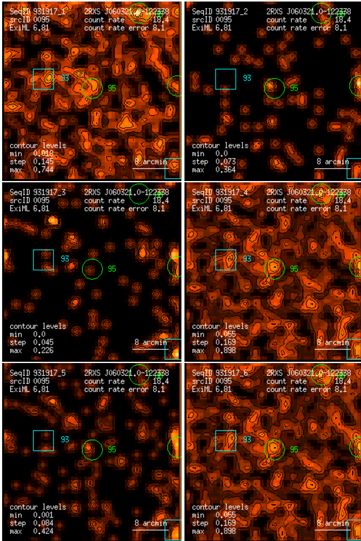
Figure 95: RASS 931917: detection 0095: band rate images, Gaussian filter: (1) PSPC channels 11 – 41, (2) 52 – 90, (3) 91 – 201, (4) 11 – 235, (5) 52 – 201, (6) 11 – 201. Broad band rates in counts/ks. Band rate contour levels in counts/ks/arcmin 2 .
