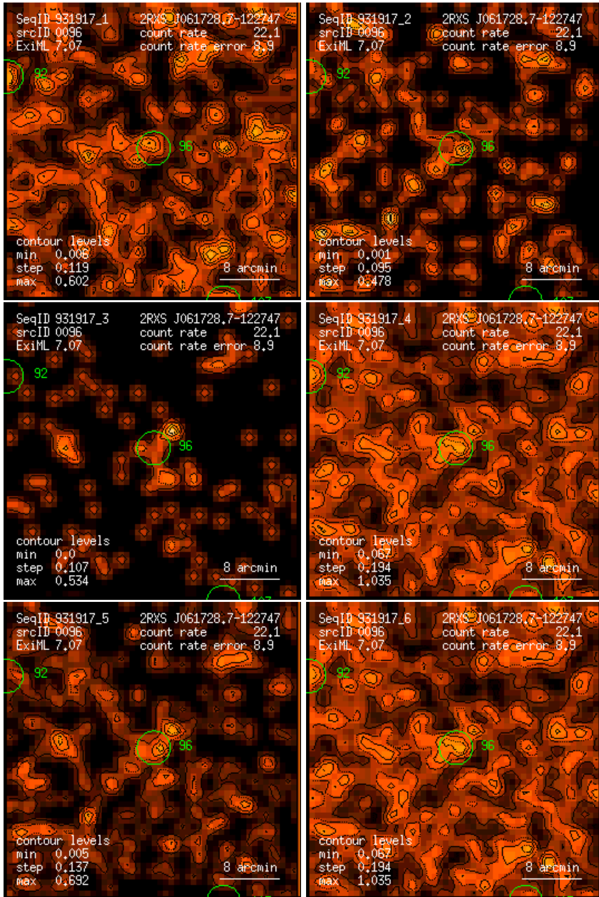
Figure 96: RASS 931917: detection 0096: band rate images, Gaussian filter: (1) PSPC channels 11 – 41, (2) 52 – 90, (3) 91 – 201, (4) 11 – 235, (5) 52 – 201, (6) 11 – 201. Broad band rates in counts/ks. Band rate contour levels in counts/ks/arcmin 2 .
