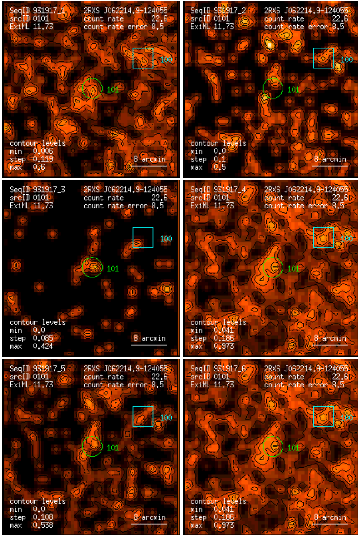
Figure 101: RASS 931917: detection 0101: band rate images, Gaussian filter: (1) PSPC channels 11 – 41, (2) 52 – 90, (3) 91 – 201, (4) 11 – 235, (5) 52 – 201, (6) 11 – 201. Broad band rates in counts/ks. Band rate contour levels in counts/ks/arcmin 2 .
