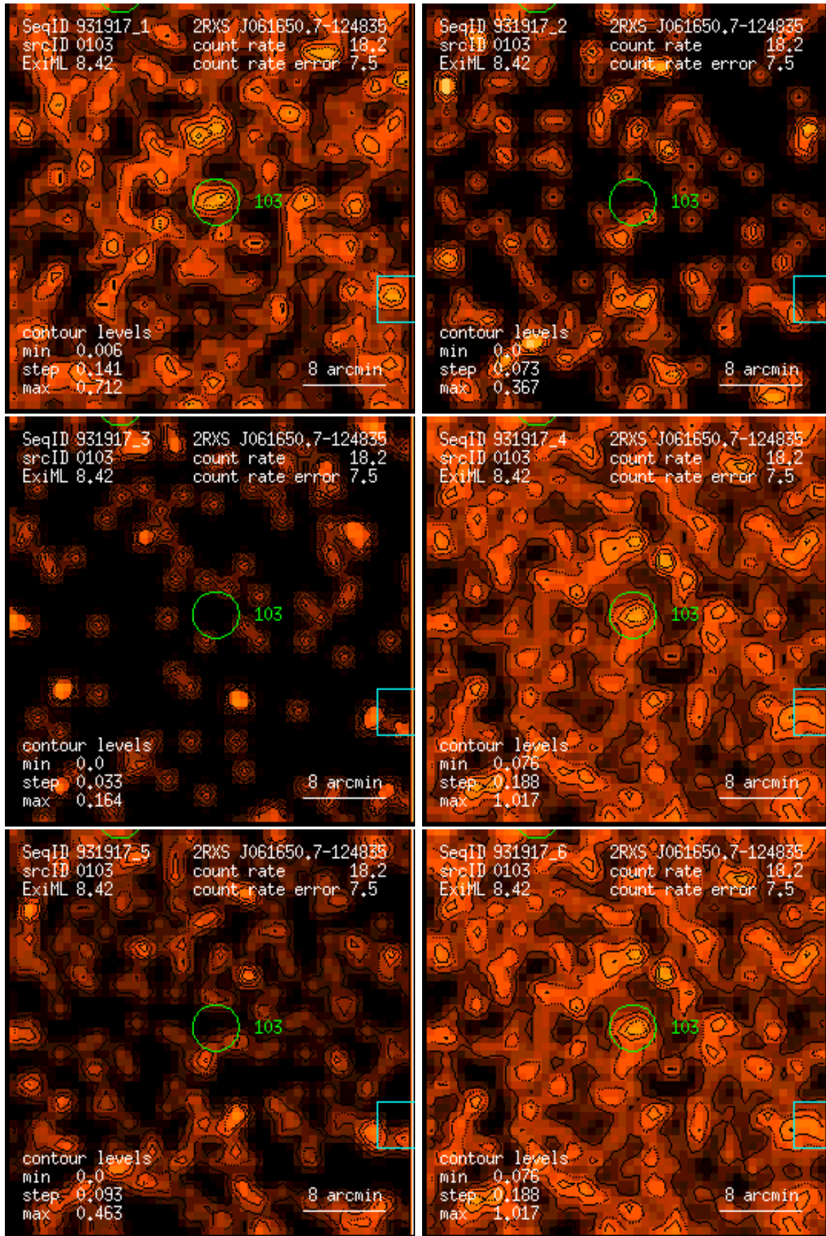
Figure 103: RASS 931917: detection 0103: band rate images, Gaussian filter: (1) PSPC channels 11 – 41, (2) 52 – 90, (3) 91 – 201, (4) 11 – 235, (5) 52 – 201, (6) 11 – 201. Broad band rates in counts/ks. Band rate contour levels in counts/ks/arcmin 2 .
