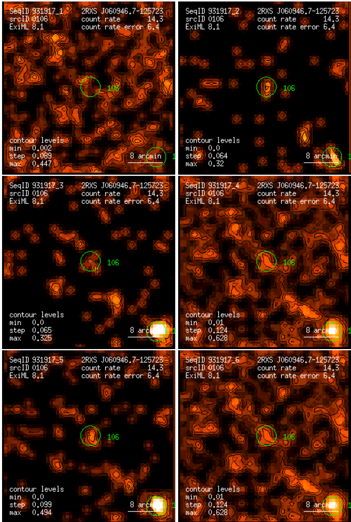
Figure 106: RASS 931917: detection 0106: band rate images, Gaussian filter: (1) PSPC channels 11 – 41, (2) 52 – 90, (3) 91 – 201, (4) 11 – 235, (5) 52 – 201, (6) 11 – 201. Broad band rates in counts/ks. Band rate contour levels in counts/ks/arcmin 2 .
